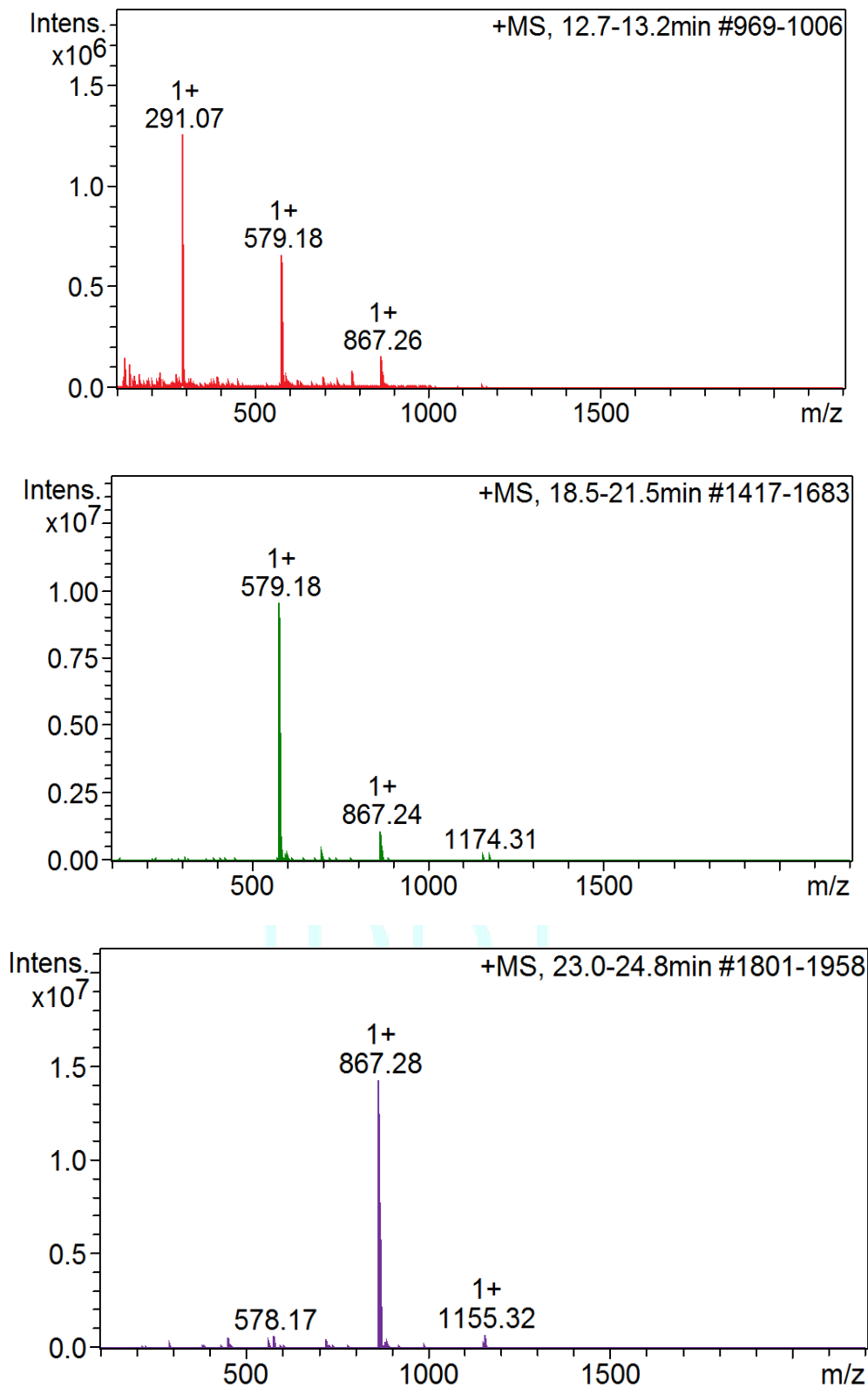
Fig. 6 : HPLC-MS chromatogram at different retention times of SF5
