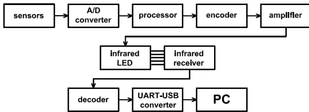
Fig. 2. The block diagram of the measuring system.
