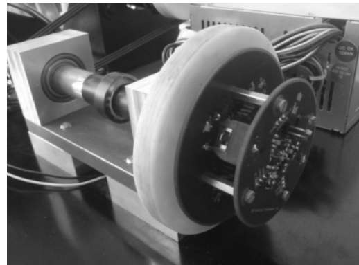
Fig. 3. System for data transport – rotating parts.
