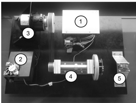
Fig. 7. Stand for equipment testing.
