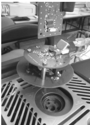
Fig. 6. Calibration - sensors of temperature in the isothermal chamber.
