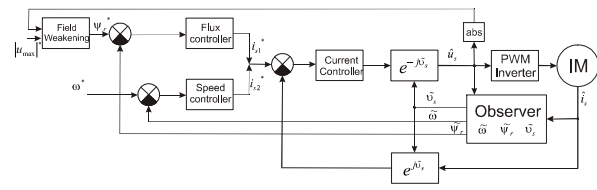
Fig. 3. Simplified flow chart of the vector control
