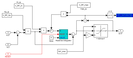
Fig. 7. Screen capture of the current controller block
