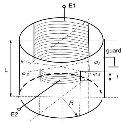
Fig. 4 Cylindrical sensor
