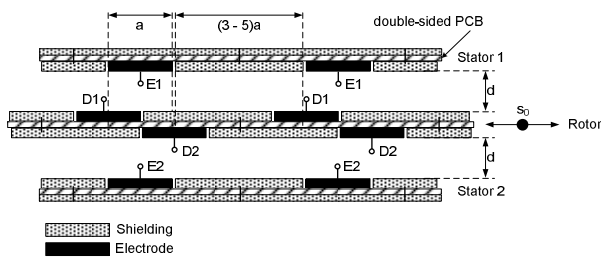
Fig.10. Front view (along the arrow) on vertically placed electrodes
