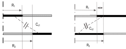
Fig. 7. Cross-capacitances of rectangular electrodes
