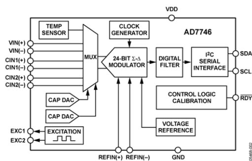
Fig. 13. Capacitance – to -Digital Converter AD 7746 by Analog Devices
