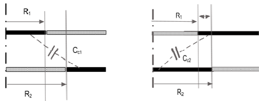
Fig. 6. Cross-capacitances of circular electrodes
