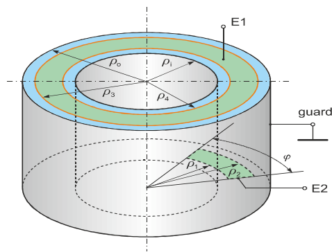
Fig.3. The archetype of the torus shaped capacitive sensor
