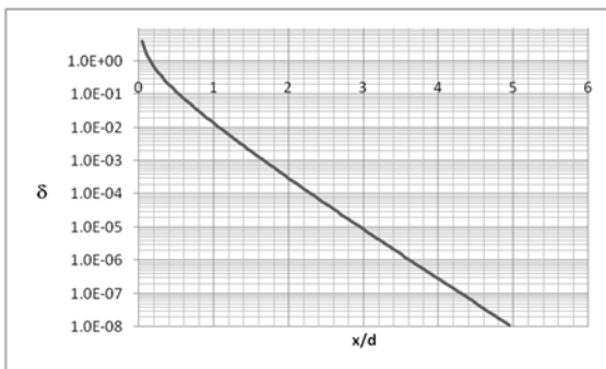
Fig. 9 a) Linearity error, single sensor
