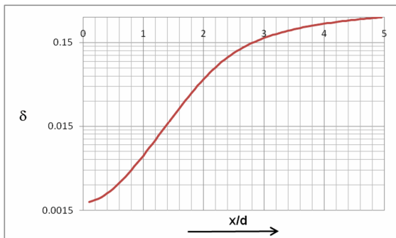
Fig. 9 a) Linearity error, single sensor
