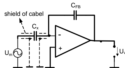
Fig. 12. Elimination of parasitic capacitances of leads.
