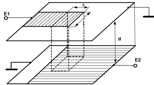
Fig. 8. Asymptotic expansion of the circular sector and ring capacitor
