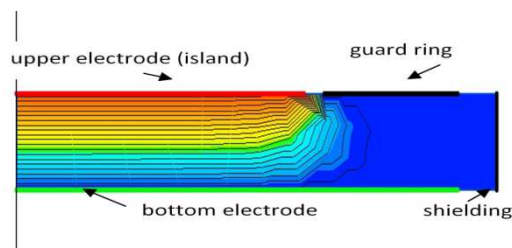
Fig. 2. Fringe field numerical model (FEM)
