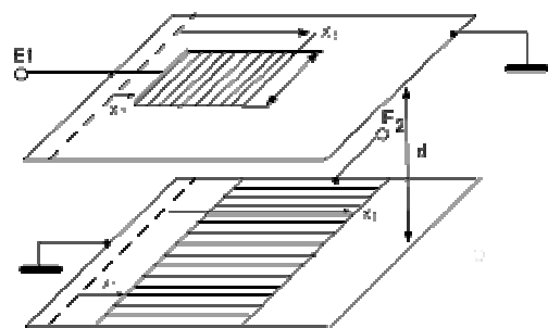
Fig. 5. Conformal mapping of the sensor in Fig. 4
