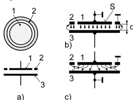
Fig. 1a). The principle of Kelvin guard ring capacitor and demonstration of independence of the capacitance on field homogeneity. The capacitance in cases b) and c) is equal
