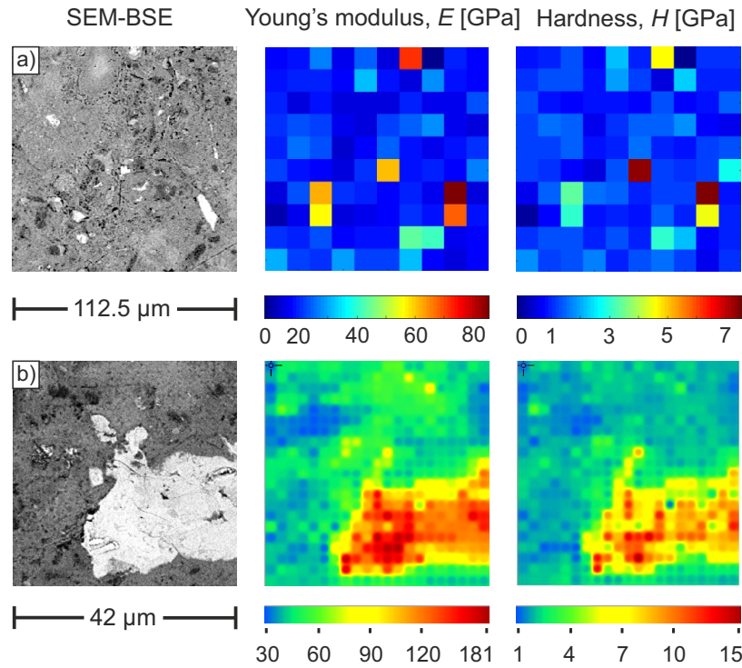
FIGURE 2. SEM-BSE image, Young's modulus, Hardness maps measured by a) NI b) XPM.
