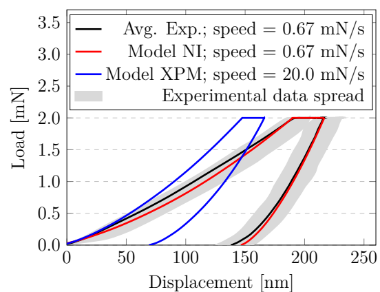
FIGURE 5. Calculated responses of NI and XPM loading with rate dependent viscoplastic model.
