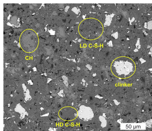
FIGURE 1. Typical SEM-BSE image of cement paste showing individual phases.
