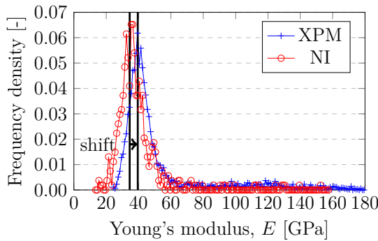
FIGURE 3. Frequency plots of NI and XPM with highlighted shift of the main peak.
