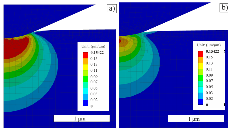
FIGURE 4. Equivalent von Mises strain under the tip at the end of loading a) at time = 3 s, speed = 0.67 mN/s (NI) b) at time = 0.1 s, speed = 20 mN/s (XPM).
