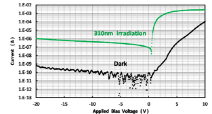
Fig.5 Dark current and UV(310nm)photo current of this device.
