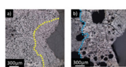
Fig.2 Microstructures of iron ore sinter reduced with high hydrogen concentration under: a) atmospheric pressure and b) 3 atm.
