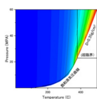
Fig.2 Estimated pH value of subcritical /supercritical fluid
