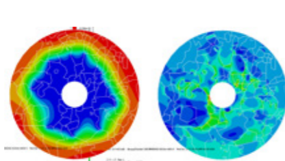
Fig.2 Simulation results of Temperature distribution (left) and stress distribution (right) when center borehole of granite is cooled from 600°C to 450°C.
