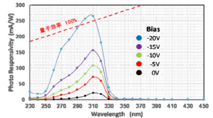
Fig.4 The comparison of spectral responsivities under various reverse bias.
