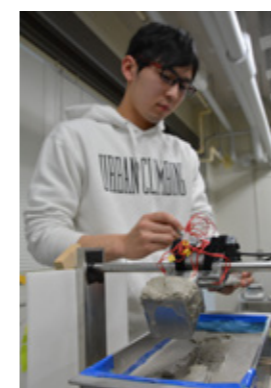
Fig.4 Bucket excavation experiment of the soil in water
