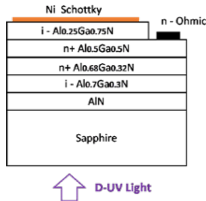
Fig.3 Device structure of the 310nm photodetector.
