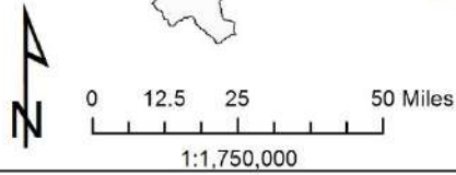
Figure 3-21. Gross isopach map of the Newburg sandstone (NBRG).
