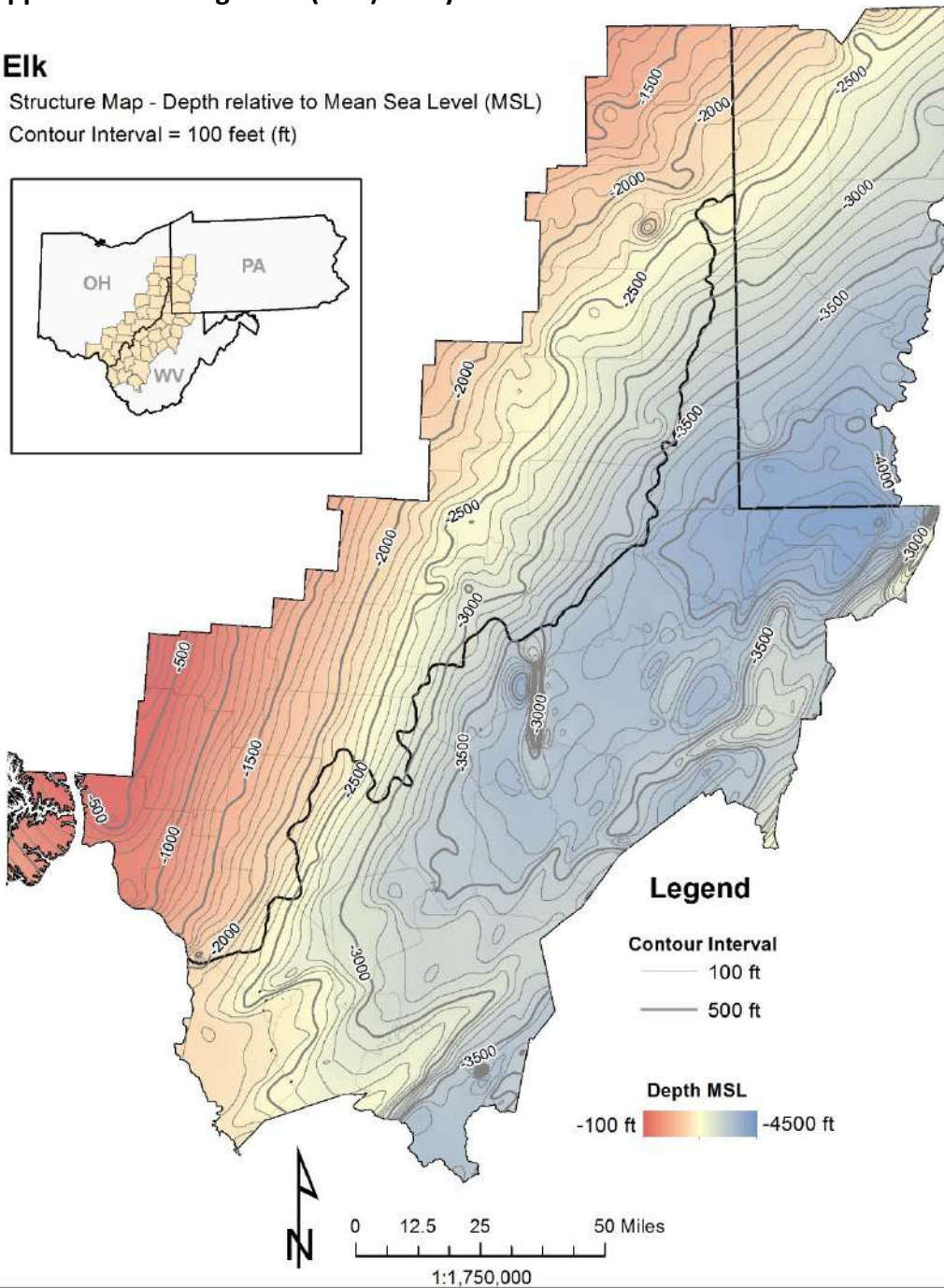
Figure 3-13. Structure contour map on top of the Elk Group (E4-E1 interval).
