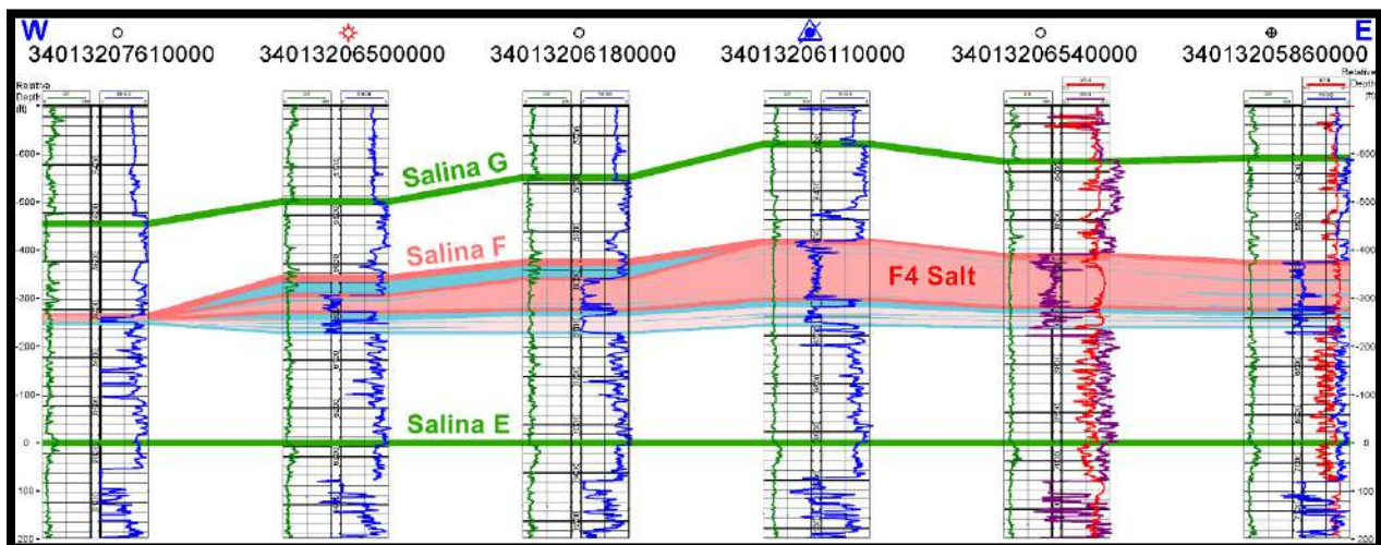
Figure 4-24. Dip (west-east) cross section through the F4 Salt in Area 3 using geophysical log control.
