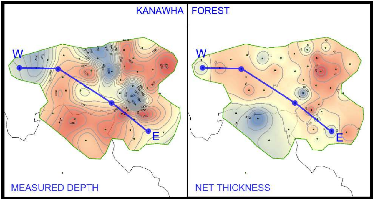
Figure 5-64. Measured depth (ft) to the Newburg sandstone (left) and net thickness (ft) (right) in Kanawha Forest Field. Cross section location shown in blue; green dots represent well control.
