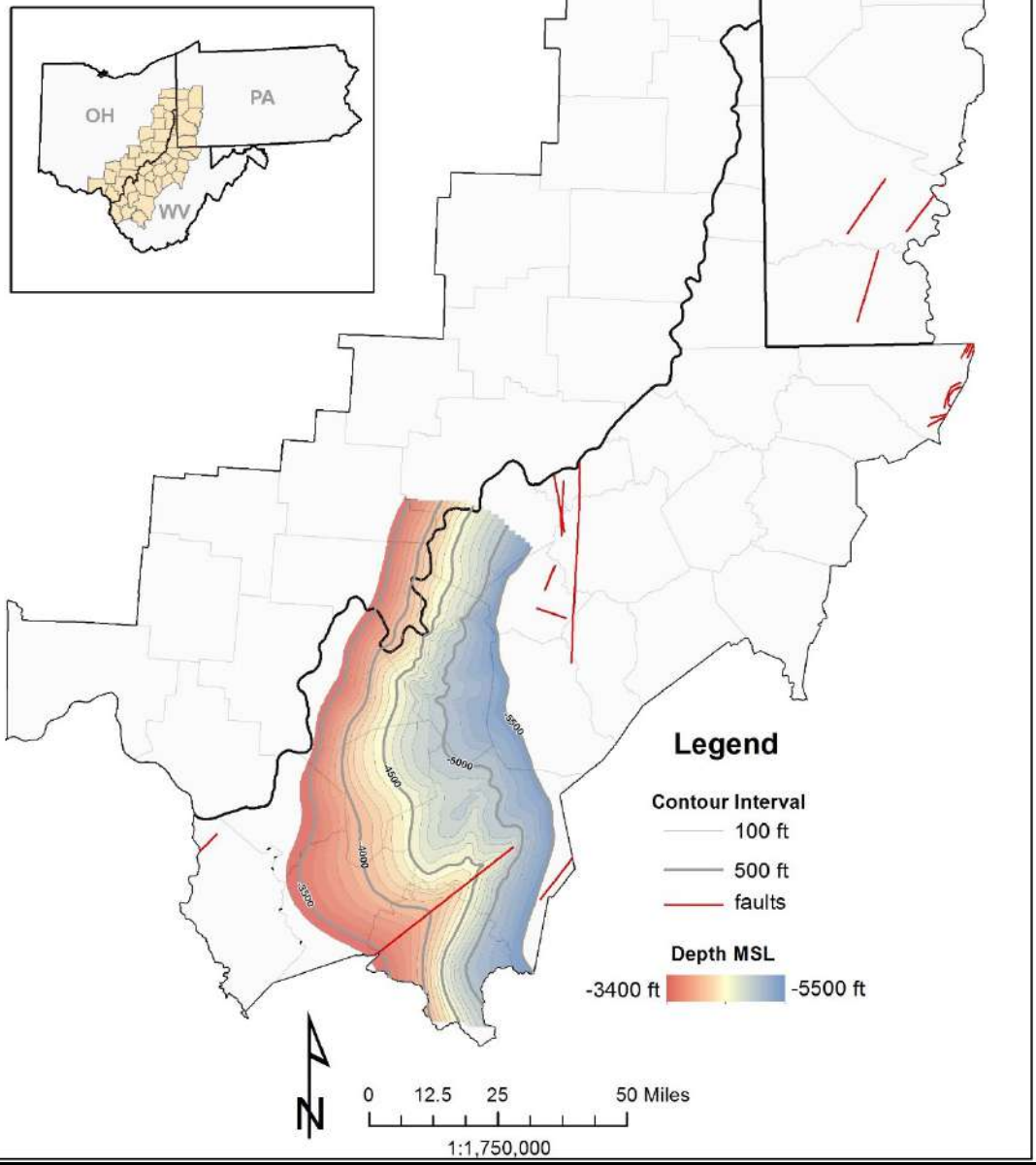
Figure 3-20. Structure contour map on top of the Newburg sandstone (NBRG).
