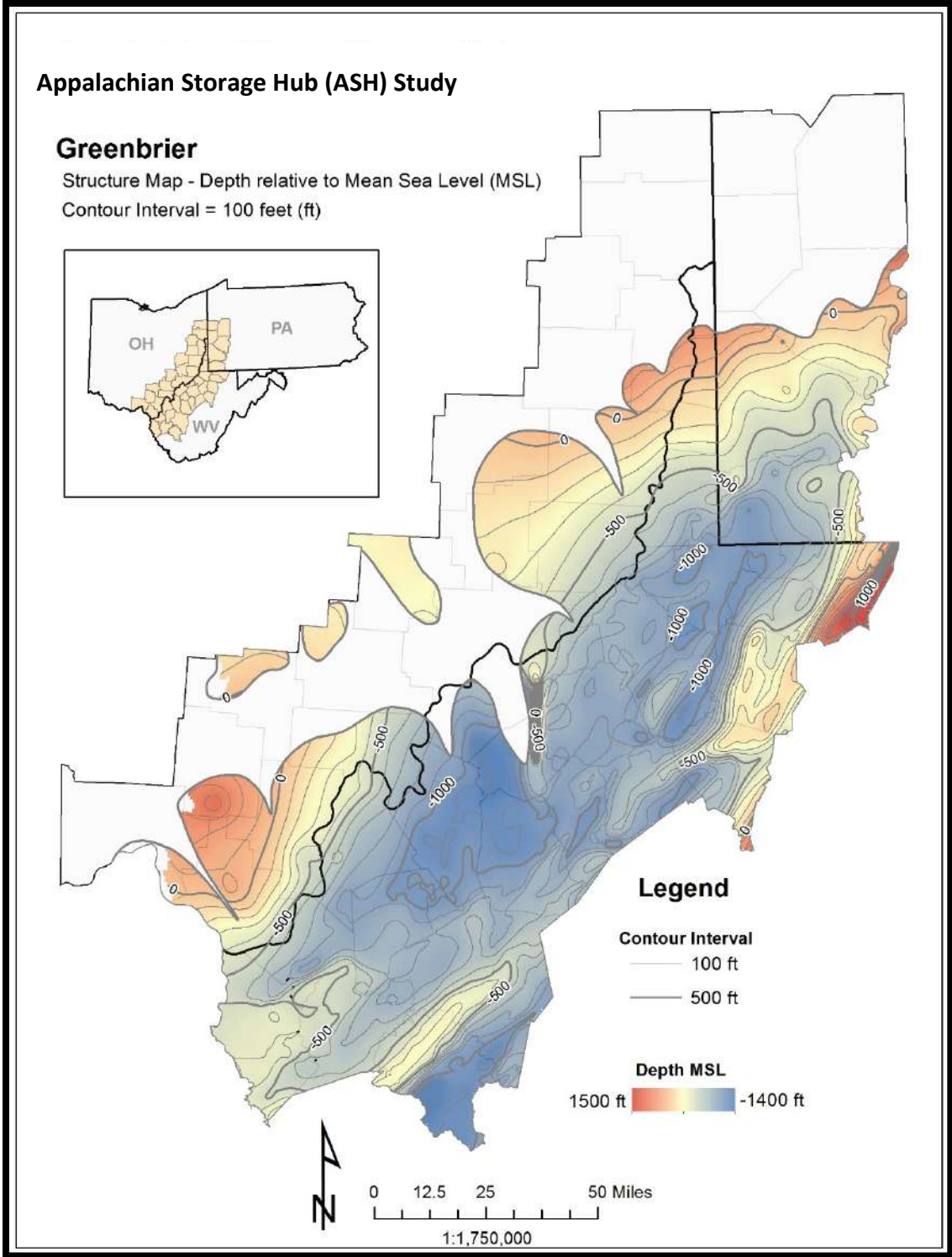
Figure 3-5. Structure contour map on top of the Greenbrier Limestone (GRNB) interval. Subcrop from Rice and Schwietering (1988).
