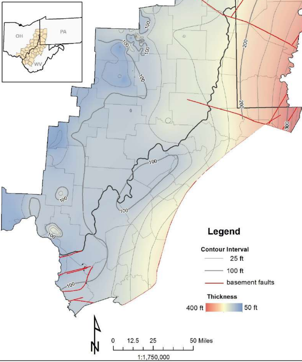
Figure 3-25. Gross isopach map of the Rose Run-Gatesburg (RSRN) interval.
