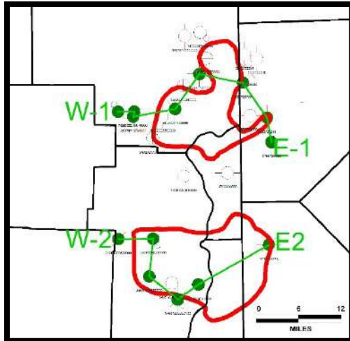
Figure 5-11. Location of cross sections through the Salina F4 Salt along dip in the Northern Prospect.
