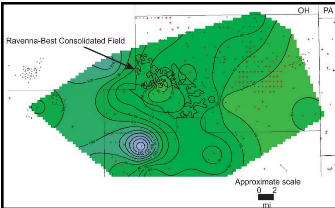
Figure 5-15. Net thickness map of the Clinton/Medina Group in the Ravenna-Best Consolidated Field (black outline). The color-ramped grid varies from green (thin areas) to purple (thick areas), and the contour interval is 10 ft.
