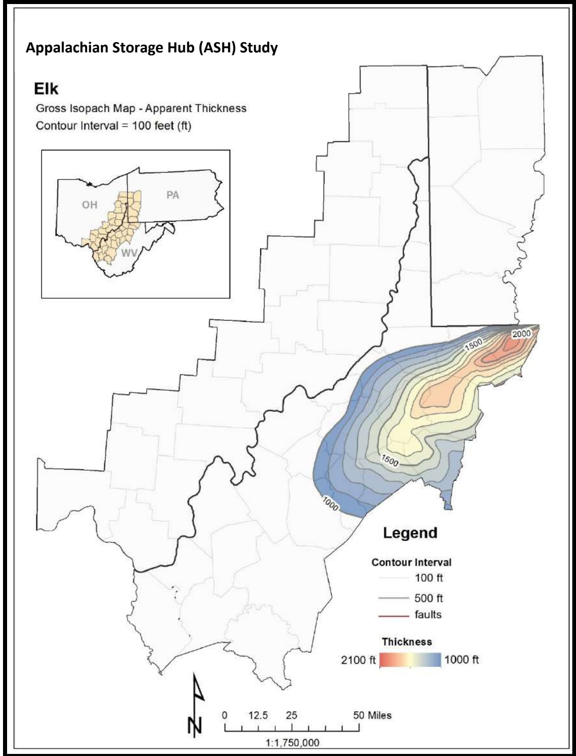
Figure 3-15. Gross isopach map of the Elk Group (E4-E1 interval) in northern West Virginia.
