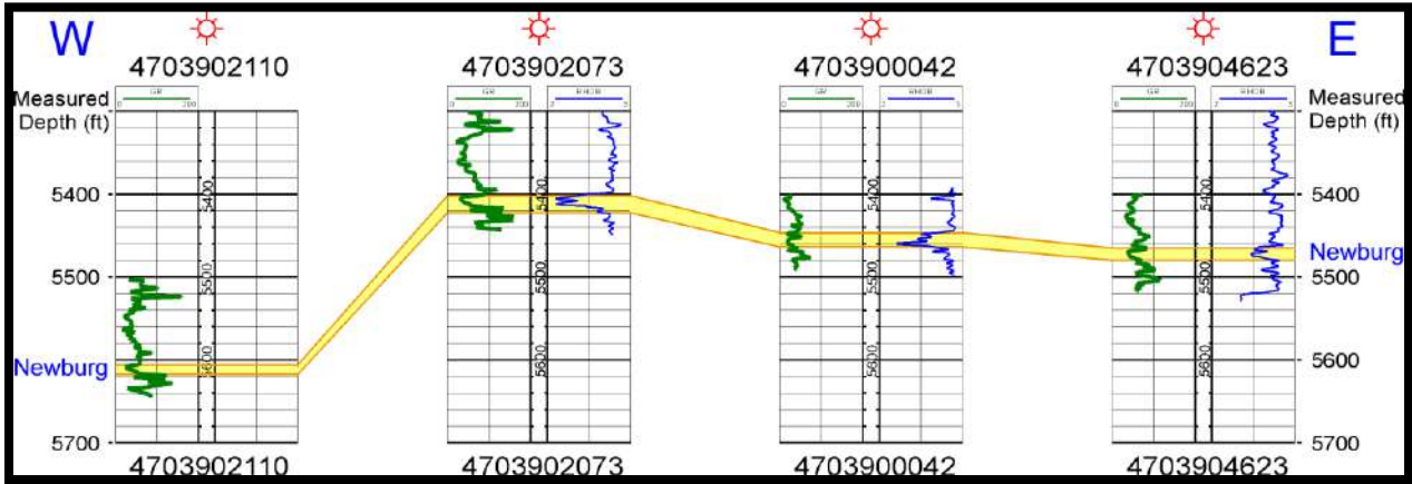
Figure 5-65. West-east cross section across Kanawha Forest Field.
