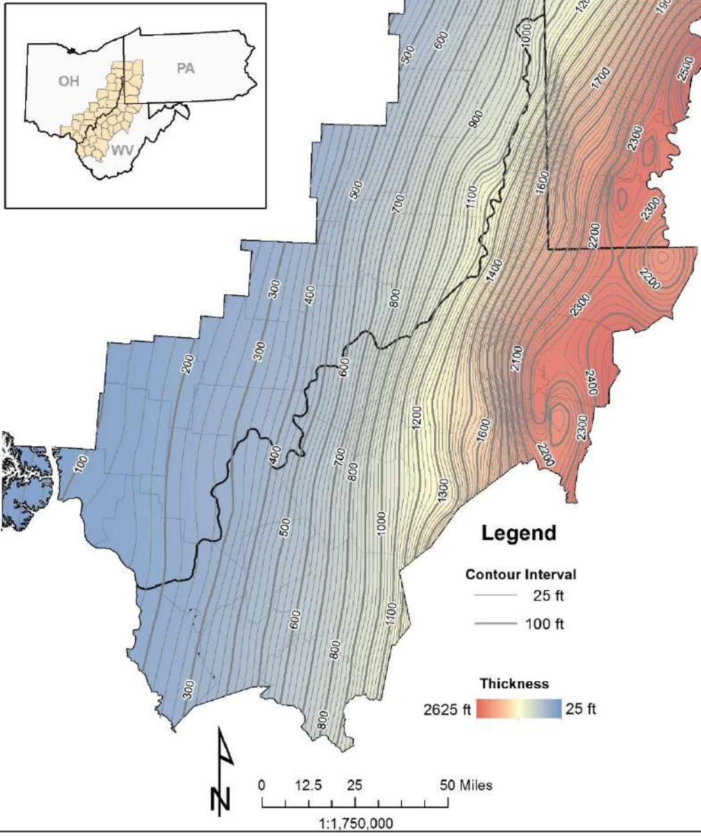
Figure 3-14. Gross isopach map of the Elk Group (E4-E1 interval) and underlying Upper Devonian clastics.
