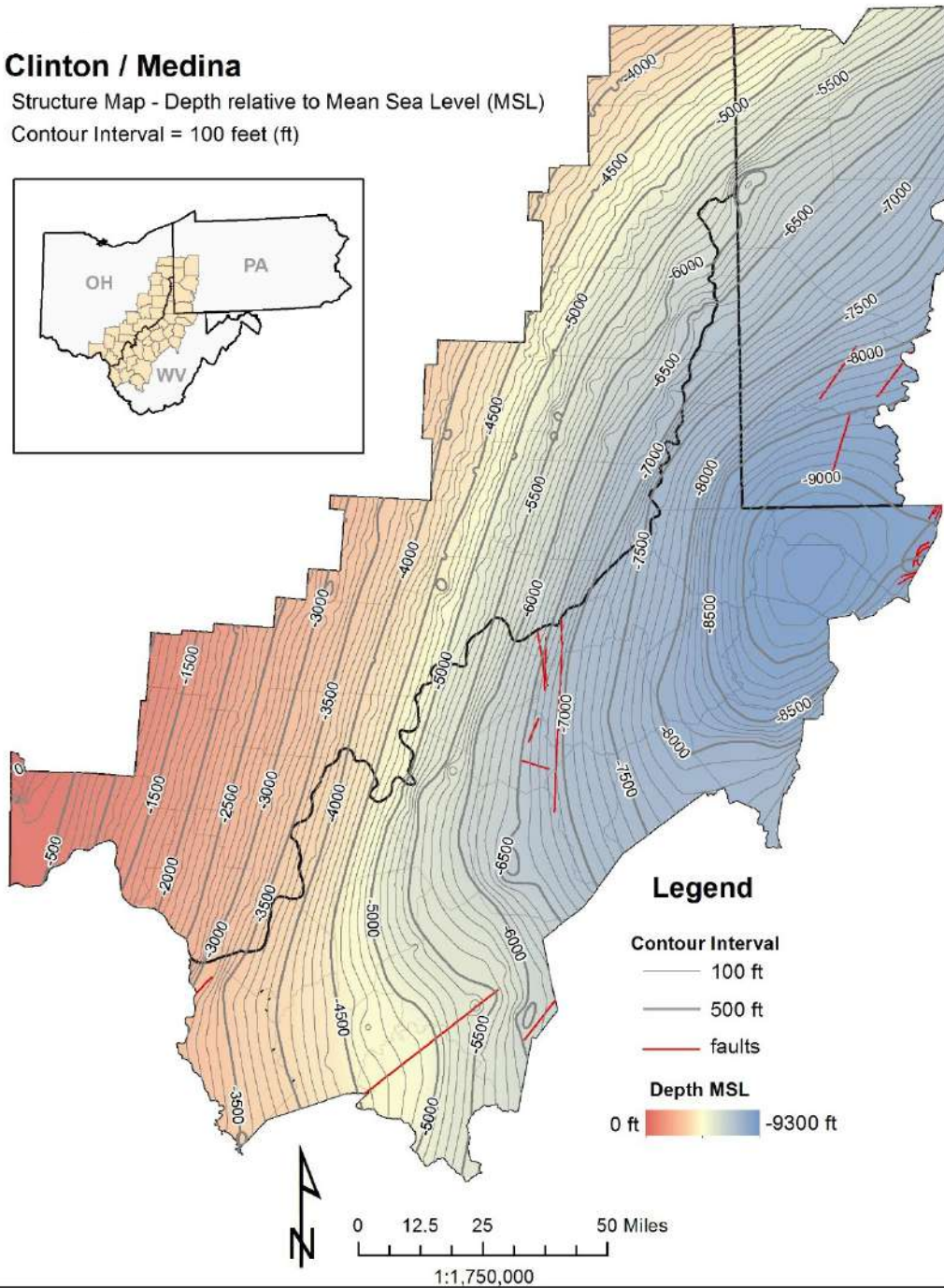
Figure 3-22. Structure contour map on top of the Clinton/Medina Group (CATG).
