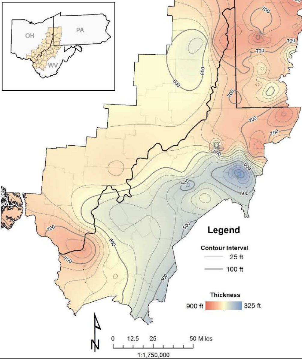
Figure 3-8. Gross isopach map of the Keener to Berea (KENR-BERE) interval.
