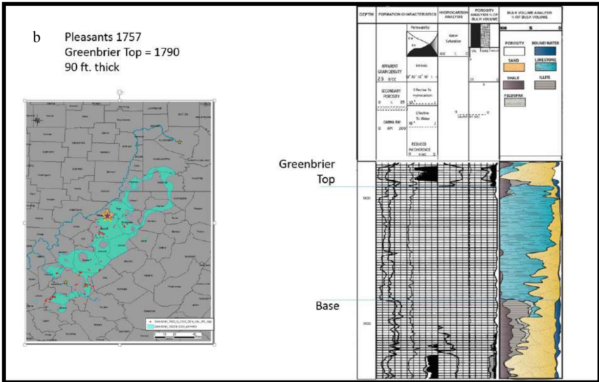
Figure 4-8. Type logs of the Greenbrier Limestone illustrating the relationship of RHOB and Pe logs to individual facies.
