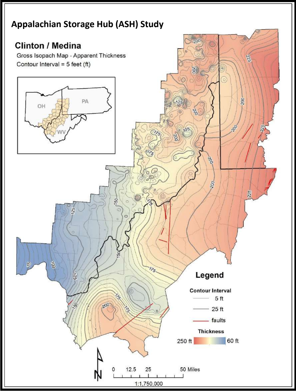
Figure 3-23. Gross isopach map of the Clinton/Medina Group (CATG).
