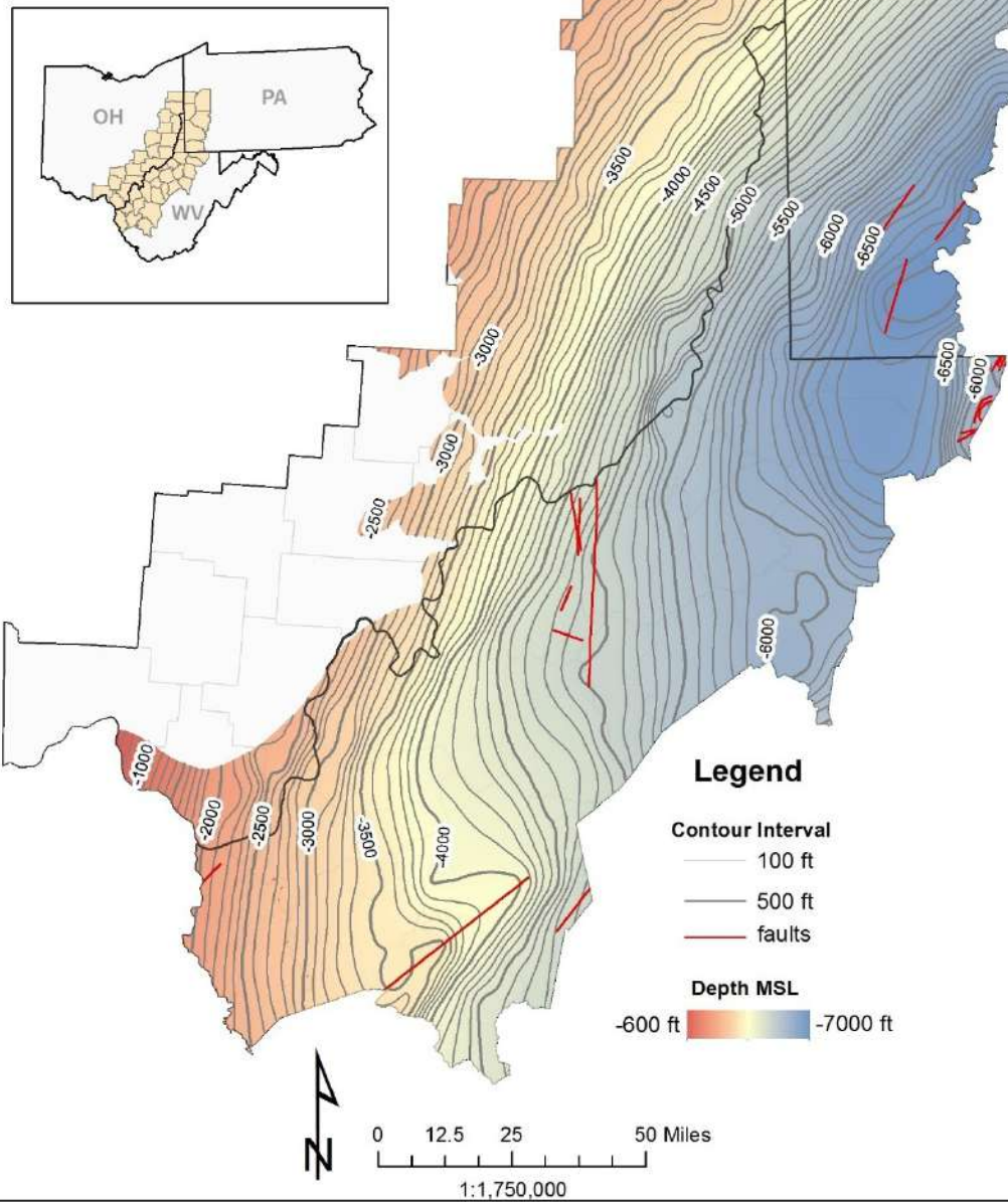
Figure 3-16. Structure contour map on top of the Oriskany Sandstone (ORSK).
