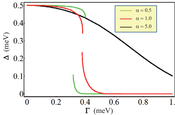
Figure 3. The solution of the gap equation (see figure 2) plotted against the Zeeman splitting \Gamma for various values of the SO coupling constant \alpha (in \text{meV \AA} ). For small values of \alpha , the superconducting gap falls discontinuously with \Gamma , but it is never strictly zero in the presence of SO coupling. Consequently, there is only a first-order-like crossover, which is a remnant of the true first-order phase transition with \Gamma for \alpha = 0 . For larger values of \alpha (black curve), the decay of the superconducting pair potential with Zeeman splitting is much slower and continuous. It falls exponentially (but is never strictly zero) only for higher fields \Gamma > 2\alpha k_F .
