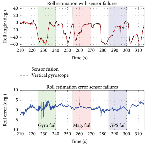
FIGURE 6: Sensor fusion with no failure, GPS failure, rate gyroscope failure, and magnetometer failure.
