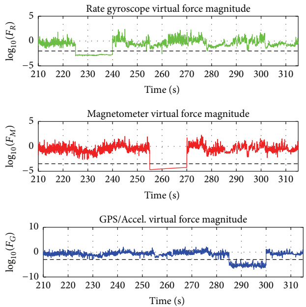
FIGURE 7: "Virtual Force Field" based failure detection signal.
