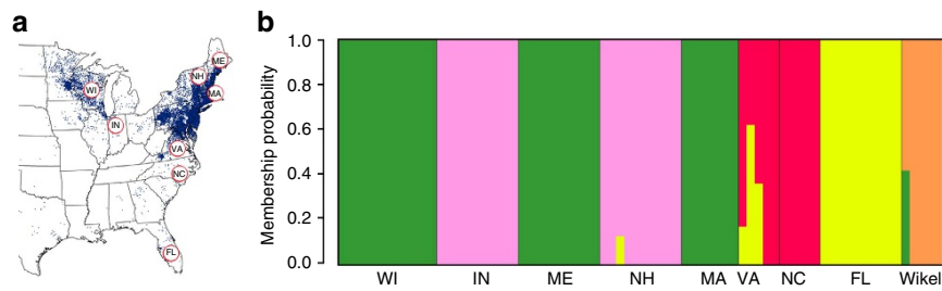
Figure 6 | Population structure of Ixodes scapularis across North America. (a) Tick sampling sites in Indiana (IN), Massachusetts (MA), Maine (ME), North Carolina (NC), New Hampshire (NH), Wisconsin (WI), Florida (FL) and Virginia (VA) overlaid against reported Lyme disease cases in 2012 (modified from CDC: http://www.cdc.gov/lyme/stats/maps/map2012.html ); (b) Membership probabilities in bar plots for individual I. scapularis comprising different clusters and showing separation of genetic groups based on 34,693 RADtag SNP markers. SNP, single-nucleotide polymorphism; WK, I. scapularis WIKEL reference strain.
