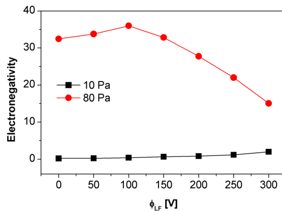
Figure 5: Electronegativity of classical dual-frequency discharges, operated at 1.937 MHz + 27.12 MHz, as a function of the low-frequency voltage amplitude, \Phi_{LF} , at different pressures (10 Pa and 80 Pa). \Phi_{HF}=300 V at 10 Pa and \Phi_{HF}=100 V at 80 Pa.
