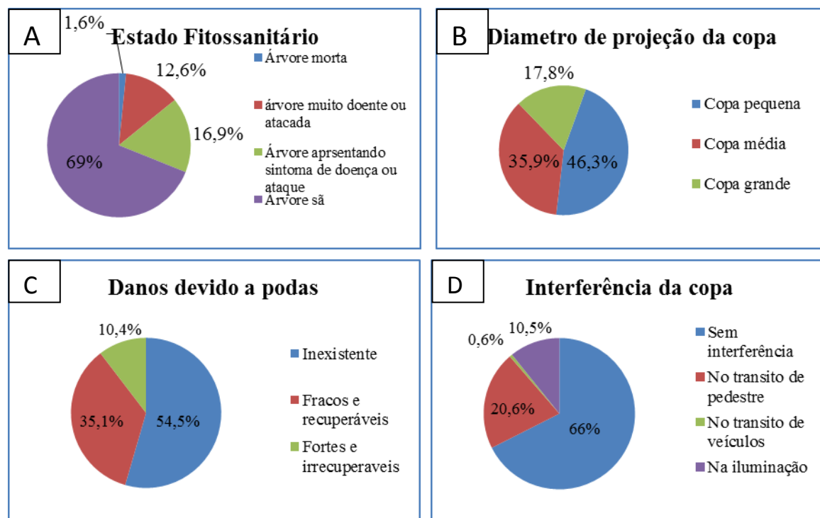
Figure 2. Appearance of trees in the neighborhoods of the urban area of the city of Timon - MA, as (the) plant health (A); diameter of the canopy projection (B); damage due to cuttings (C); interference of the crown (D).
