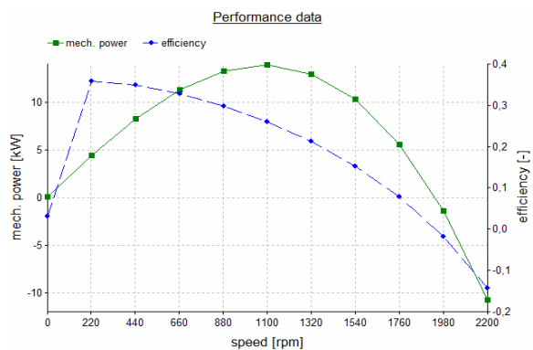
Figure 6. Influence of rotation on mechanical power and efficiency for the Amazon engine optimized by PROSA.
