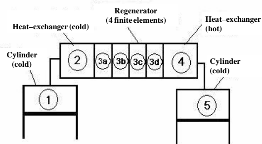
Figure 2. Division of the Stirling engine in different volumes or finite element to the PROSA software (Adapted from Thomas, 2003).
