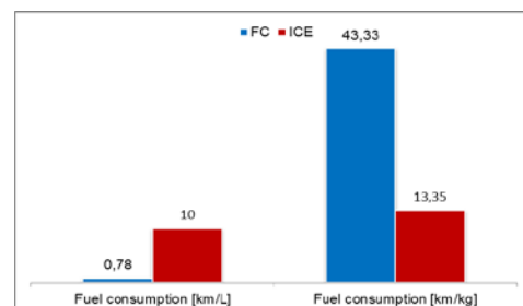
Figure 14. Fuel consumption of the urban cycle.
