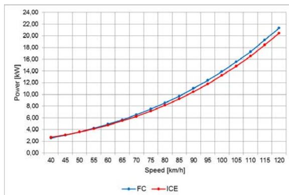
Figure 7. Power curve.
