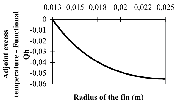
Figure 2. Adjoint excess temperature versus radius of the fin – Functional Q_h .
