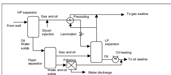
Figure 8. Scheme of a gas-oil separation plant.
