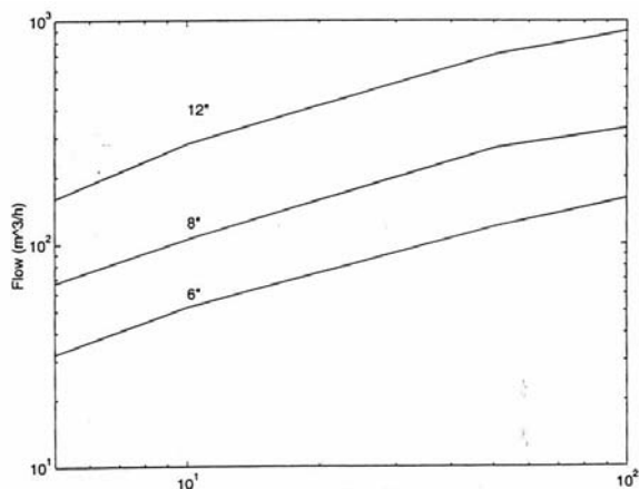
System pressure drop (kPa/100 m) Figure 6. Typical two-phase pressure drop (well fluids with low/medium Gas-Oil Ratio).
