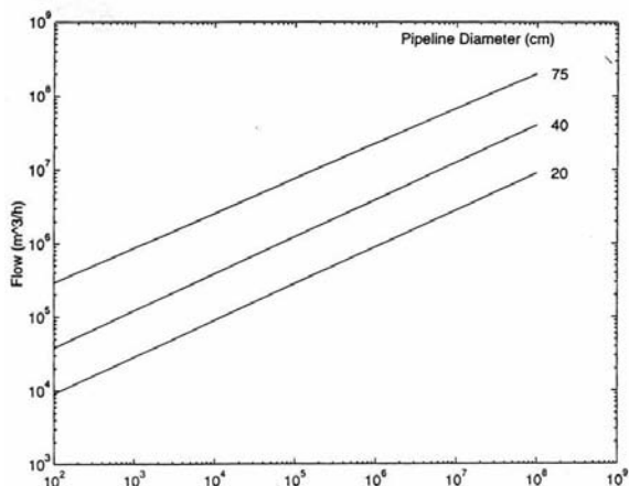
P_1^2 - P_2^2 (kPa 2 /km) Figure 5. Gas pipeline sizing.
