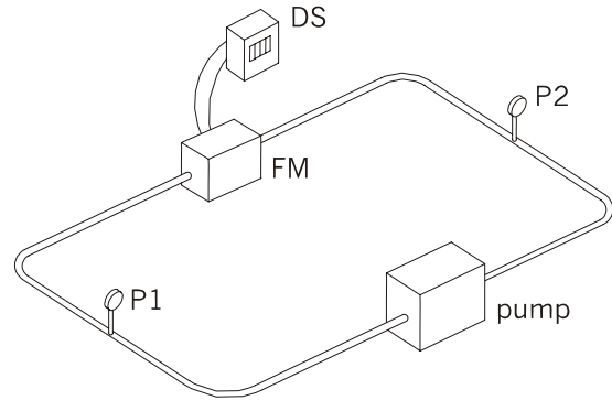
Figure 11. Experimental loop of DC electromagnetic pumps to dynamic mercury fluid flow.
