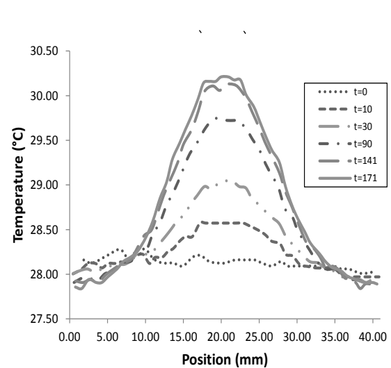
Figure 6. Temperature distribution along a straight line at the front face.
