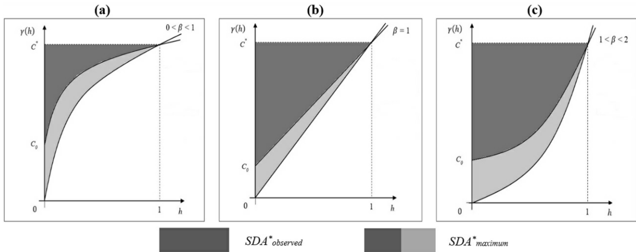
Figure 2: Equivalent observed and maximum spatial dependence areas for the power model with (a) 0 < \beta < 1 ; (b) \beta = 1 ; (c) 1 < \beta < 2 .
