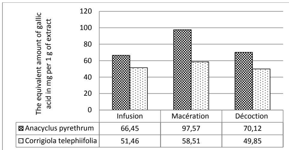
Fig. 3: Determination of polyphenols from aqueous plant extracts
