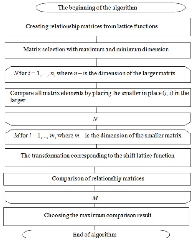
Figure 6 – General algorithm for comparing lattice functions
