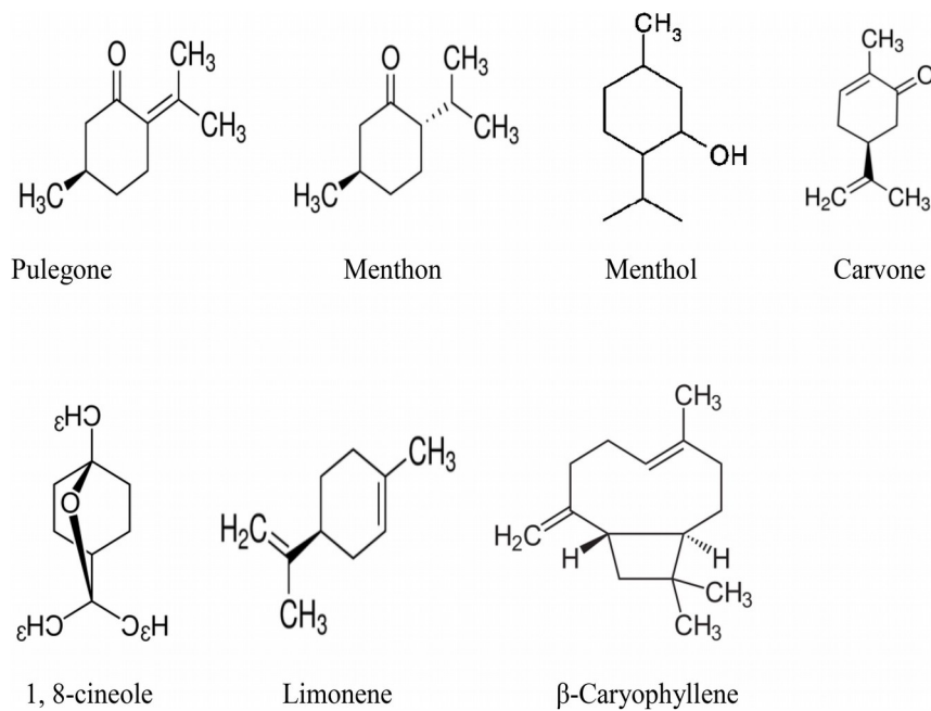
Fig. 1 Chemical structure of main compounds of Mentha species essential oils
