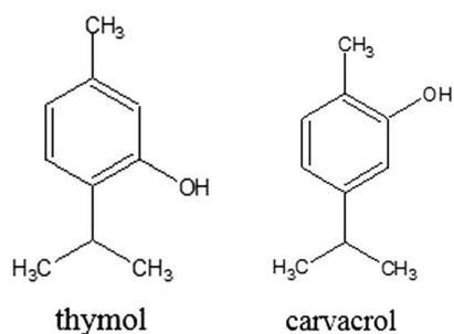
Fig. 2 Chemical structure of main compounds of Thymus species essential oils (Muchebleled, J., Deweer, C., Sahmer, K., Halama, P., 2018)
