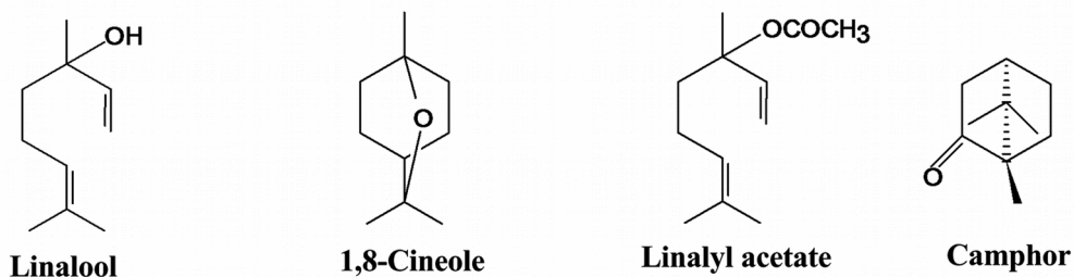
Fig. Chemical structure of main compounds of Lavandula species essential oils (Aprotosoaie, A.C. et al., 2017).
