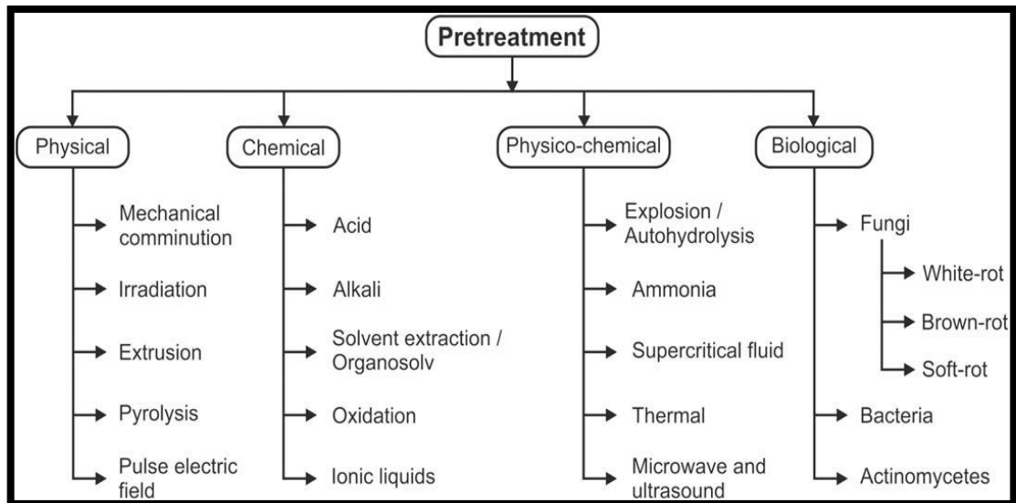
Figure 3. Scheme for various pretreatment of biomass[30].
