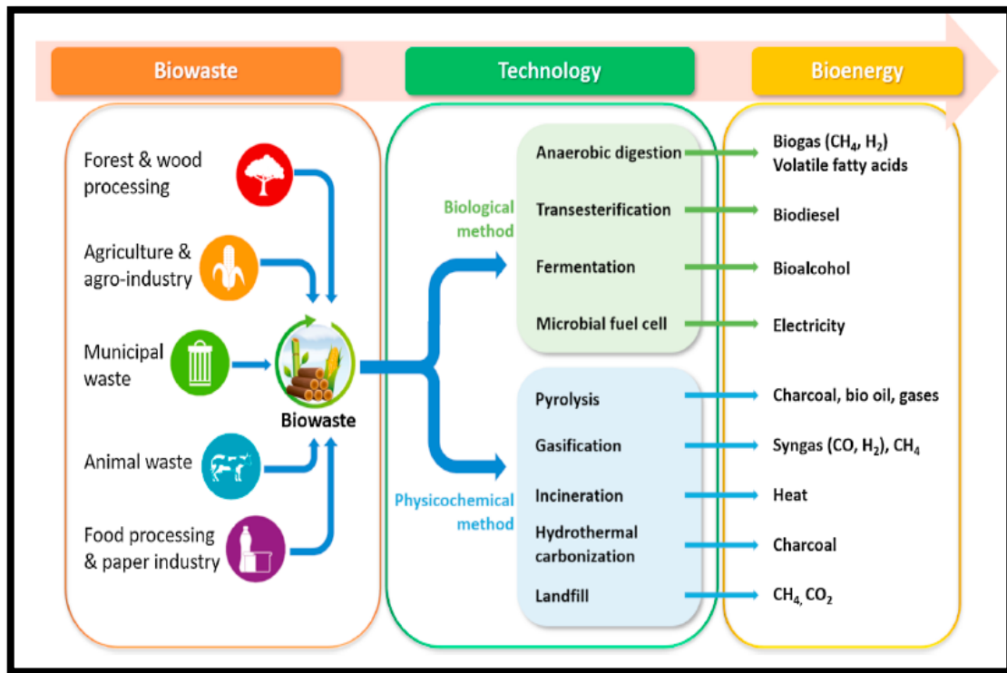
Figure 1. Scheme showing the production of biofuels from various bio-waste [13].
