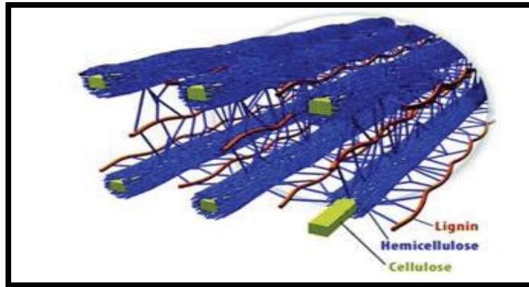
Figure2. Structure of lignocelluloses biomass [17].
