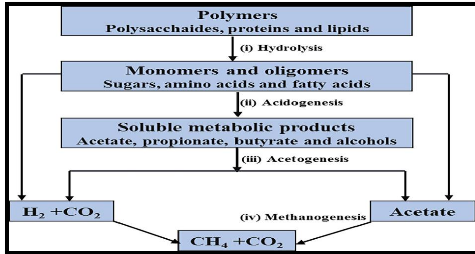
Figure 5. Anaerobic digestion for production biogas[73].
