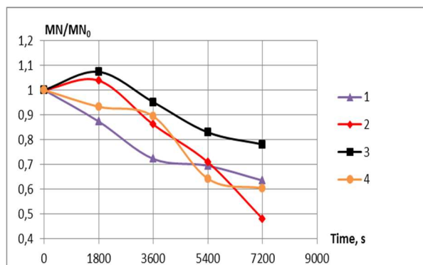
Figure. 3: Character of dependence of ratio MN / MN_0 on duration of cleaning domestic wastewater in presence of gases of various nature: 1-N 2 ; 2-O 2 ; 3-N 2 +O 2 ; 4-Air
