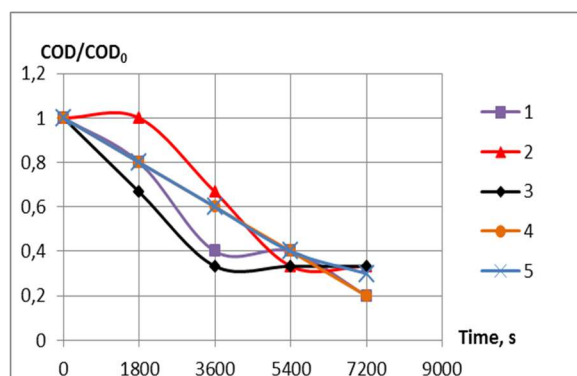
Figure 2. Character of sound and chemical dependence of ratio COD/COD 0 on duration of cleaning domestic wastewater under different experimental conditions: 1- N 2 /US; 2-O 2 /US; 3-(N 2 +O 2 )/US; 4-Air/US; 5-US
