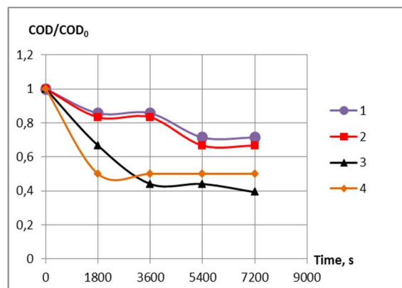
Figure 1. Character of dependence of ratio COD/COD 0 on duration of cleaning domestic wastewater under different experimental conditions: 1-N 2 ; 2-O 2 ; 3-N 2 +O 2 ; 4-Air
