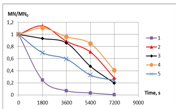
Figure 4. Character of sound and chemical dependence of ratio MN / MN_0 on duration of cleaning domestic wastewater under different experimental conditions: 1- N_2/US ; 2- O_2/US ; 3- (N_2+O_2)/US ; 4- Air/US ; 5- US ;
