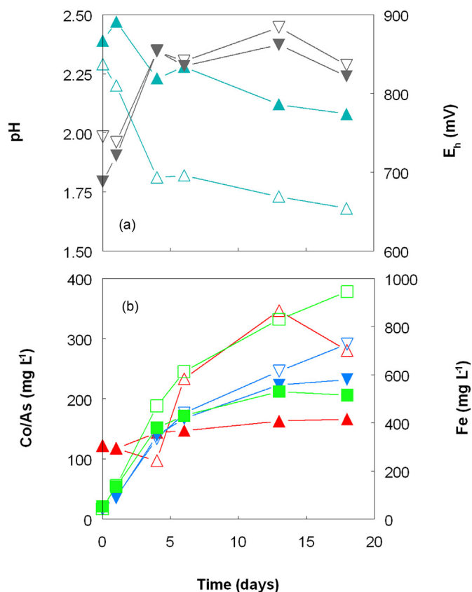
Fig. 2. Changes in (a) pH ( \blacktriangle , \triangle ) redox potentials ( \blacktriangledown , \triangledown ) and (b) concentrations of soluble cobalt ( \blacktriangledown , \triangledown ), iron ( \blacktriangle , \triangle ) and arsenic ( \blacksquare , \square ) during the bioleaching of Iron Mask ore in replicate bioreactors (experiment 1).
