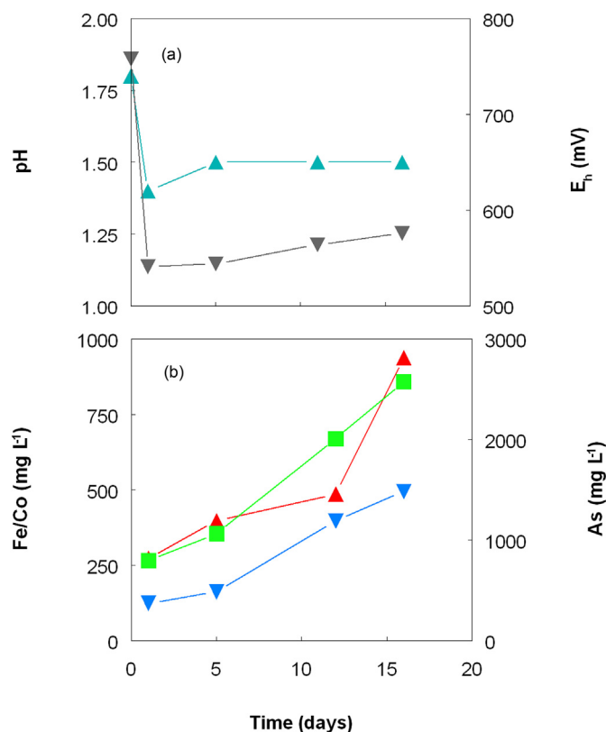
Fig. 3. Changes in (a) pH ( \blacktriangle ) redox potentials ( \blacktriangledown and \triangledown ) and (b) concentrations of soluble cobalt ( \blacktriangledown ), iron ( \blacktriangle ) and arsenic ( \blacksquare ) during the bioleaching of Bou Azzer concentrate in a replicate bioreactors.
