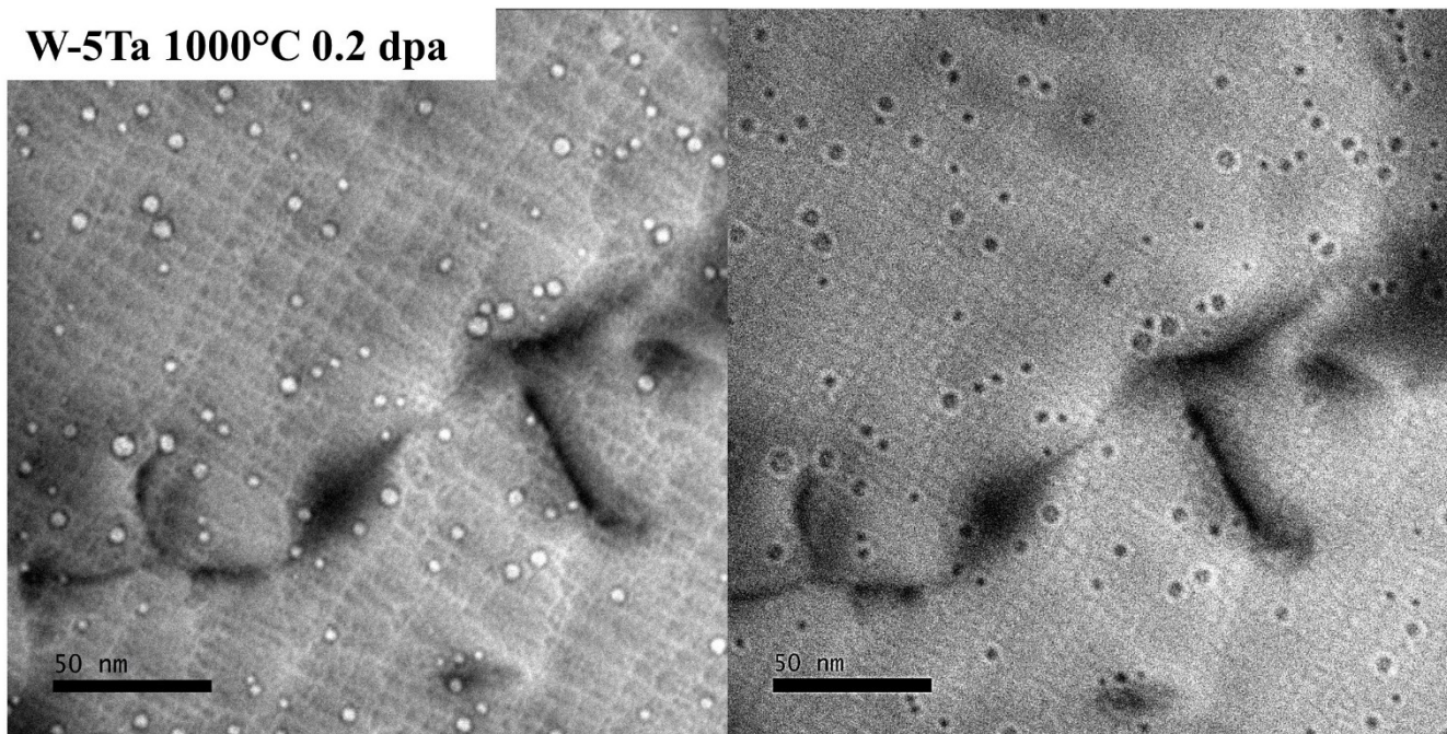
Fig. S2. Bright field TEM images of voids in W-5Ta proton-irradiated at 1000 °C and to a damage level of at 0.2 dpa. The images were taken using the out-of-focus imaging technique with the defocus value of +/-500 nm. Dislocations present in the micrographs correspond to pre-existing dislocations prior to irradiation.
