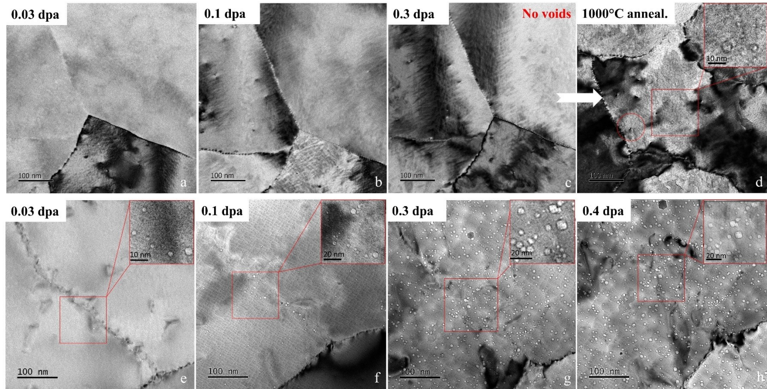
Fig. 2. In-situ observation of void growth, together with changes in void shape (insets) in W-5Ta under increasing damage levels induced by 40 keV proton bombardment at 800 °C: (a) 0.03 dpa, (b) 0.1 dpa, (c) 0.3 dpa, (d) after post-irradiation annealing at 1000 °C; and 1000 °C at 800 °C: (e) 0.03 dpa, (f) 0.1 dpa, (g) 0.3 dpa, (h) 0.4 dpa. Radiation-induced voids were not detected in the irradiated material at 800 °C, but can be seen in the same sample after post-irradiation annealing at 1000 °C.
