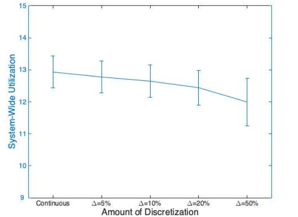
Figure 13: Average Utilization (10K Tasksets)
