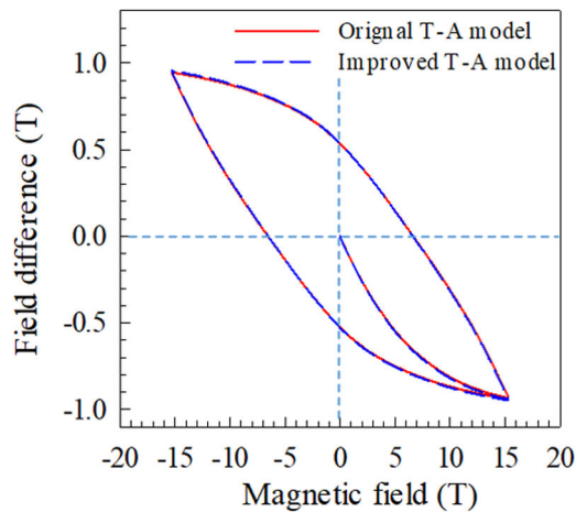
Fig. 10 Influence of SCIF during the ramping up and down cycles: x -axis is the central magnetic field of the magnet with uniform current density on REBC tapes, y -axis is the central field difference \Delta B defined in (8)
