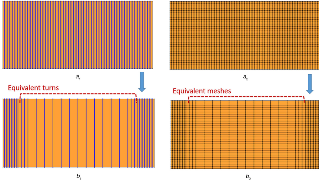
Fig. 2 2D axisymmetric T-A models for pancake coils using REBCO tapes
