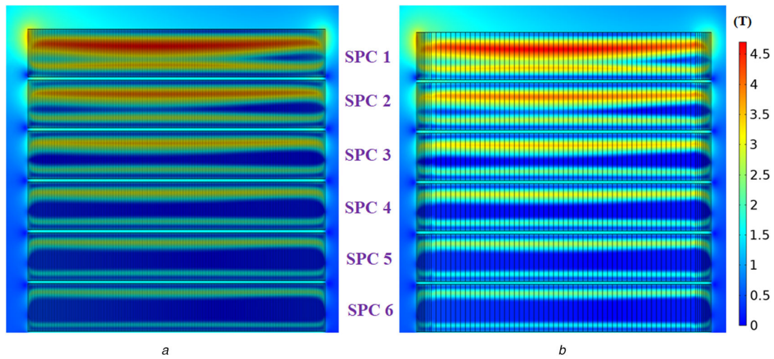
Fig. 8 Distribution of magnetic fields norm \|B\| when the transport current is ramped down to 0 A for the first time ( t = 400 s) (a) Original T-A model, (b) Improved T-A model
