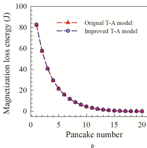
Fig. 11 Magnetisation loss of the 20 SPCs during the ramping up and ramping down operations
