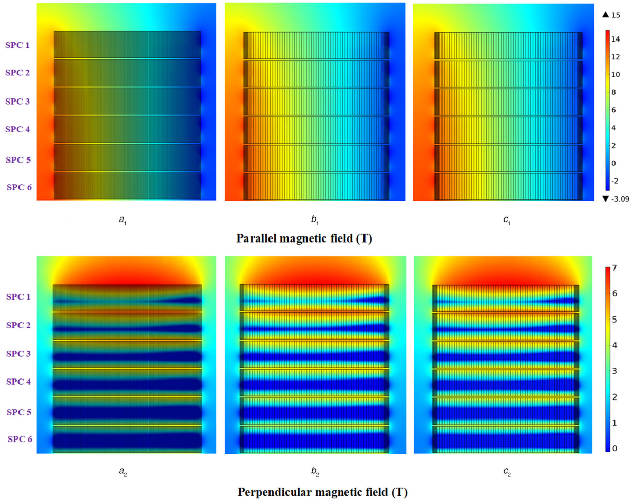
Fig. 5 Distribution of magnetic fields norm \|B\| when the transport current is ramped up to 200 A for the first time ( t = 200 s). Notice that only the top 6 pancakes are plot here, where the magnetic field have a significant variation; the following 14 pancakes are not shown ( a_1 ), ( a_2 ) Original T-A model, ( b_1 ), ( b_2 ) Improved T-A model, ( c_1 ), ( c_2 ) H-formulation model
