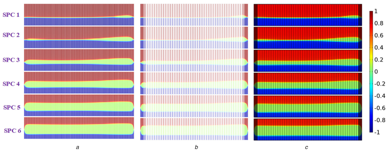
Fig. 6 Normalised current density J/J_c when the transport current is ramped up to 200 A for the first time ( t = 200 s)
