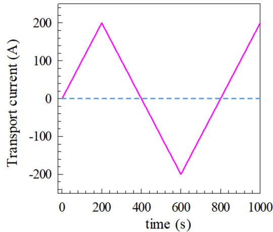
Fig. 4 Transport current of the magnet during the ramping up and down operation, ramping rate 1 A/s
