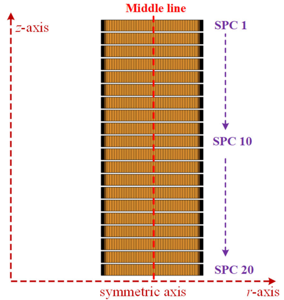
Fig. 3 2D axisymmetric T-A models for REBCO magnet with multiple coils
