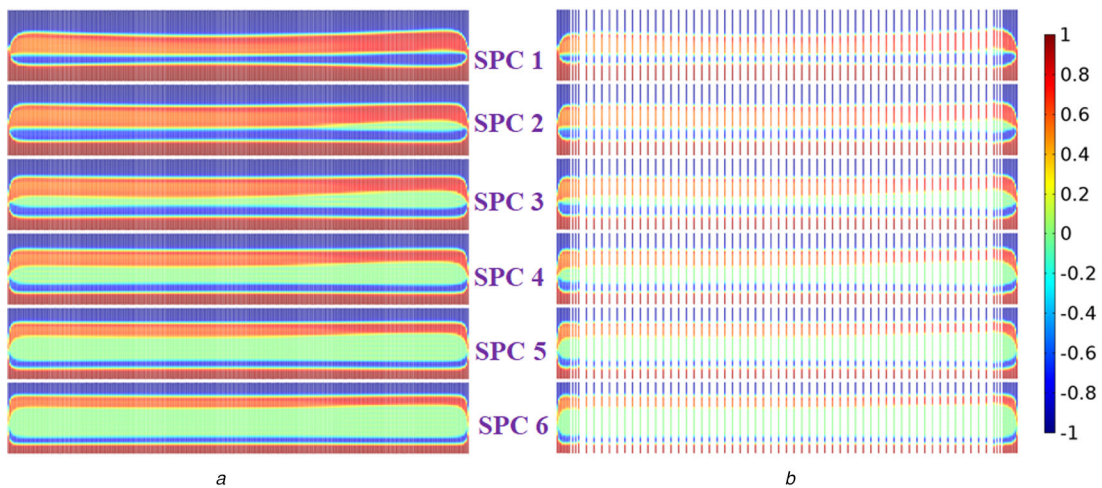
Fig. 9 Normalised current density J/J_c when the transport current is ramped down to 0 A for the first time ( t = 400 s) (a) Original model with actual turns, (b) Improved T-A model with equivalent turns. Note that current on superconducting shell (line) without thickness is plotted as tube with thickness for better visualisation
