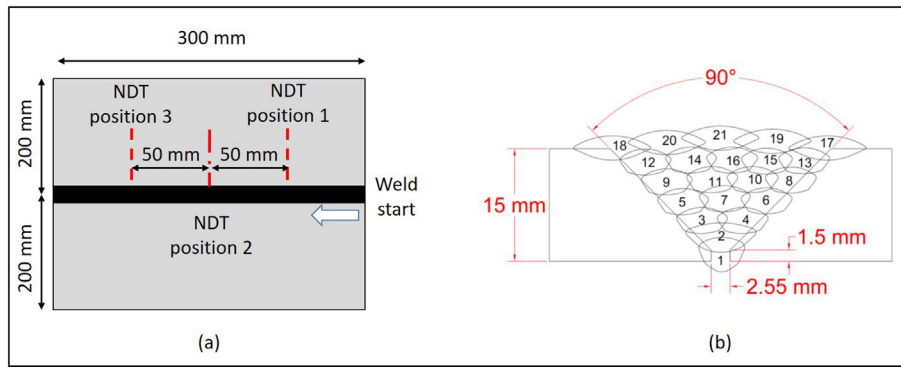
Figure 1. Sample geometry (a) and weld layout (b)
