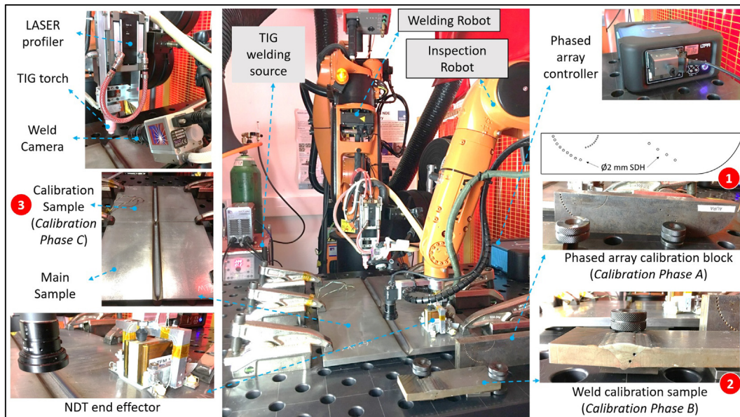
Figure 3. In-process calibration setup
