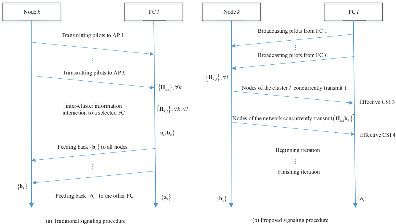
Figure 4. The signaling procedure of transceiver optimization.
