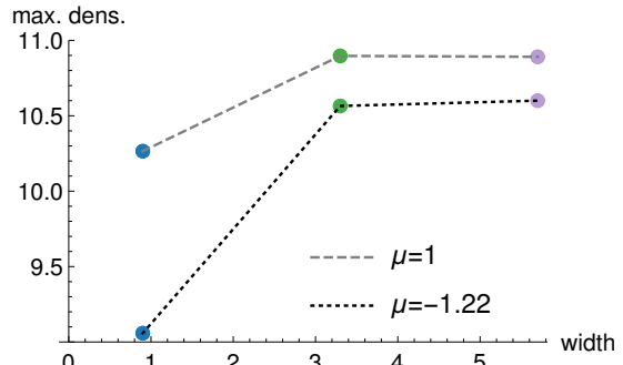
(B) Maximum agent density using the CA model with n = 60 .
