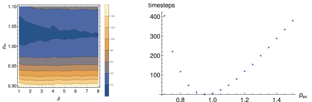
(A) The average exit time for a discrete set of \beta/p_{ex} -combinations.
