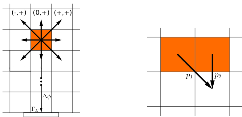
(A) Moore neighborhood and selected elements of I ; the potential \phi corresponds to the distance to the exit.
