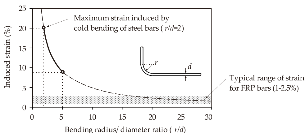
Figure 1. Induced strain values in cold-bent bars (adapted from Imjai et al. [38]).
