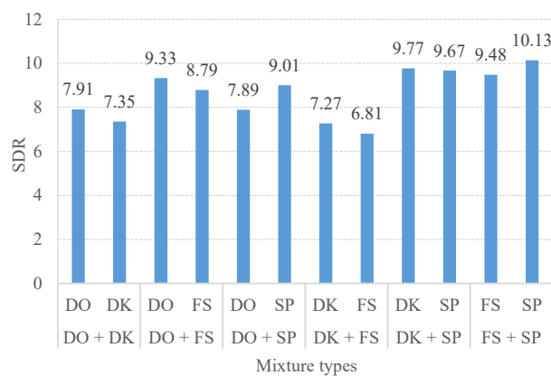
Figure 3. Average SDR results of six-mixture types.
