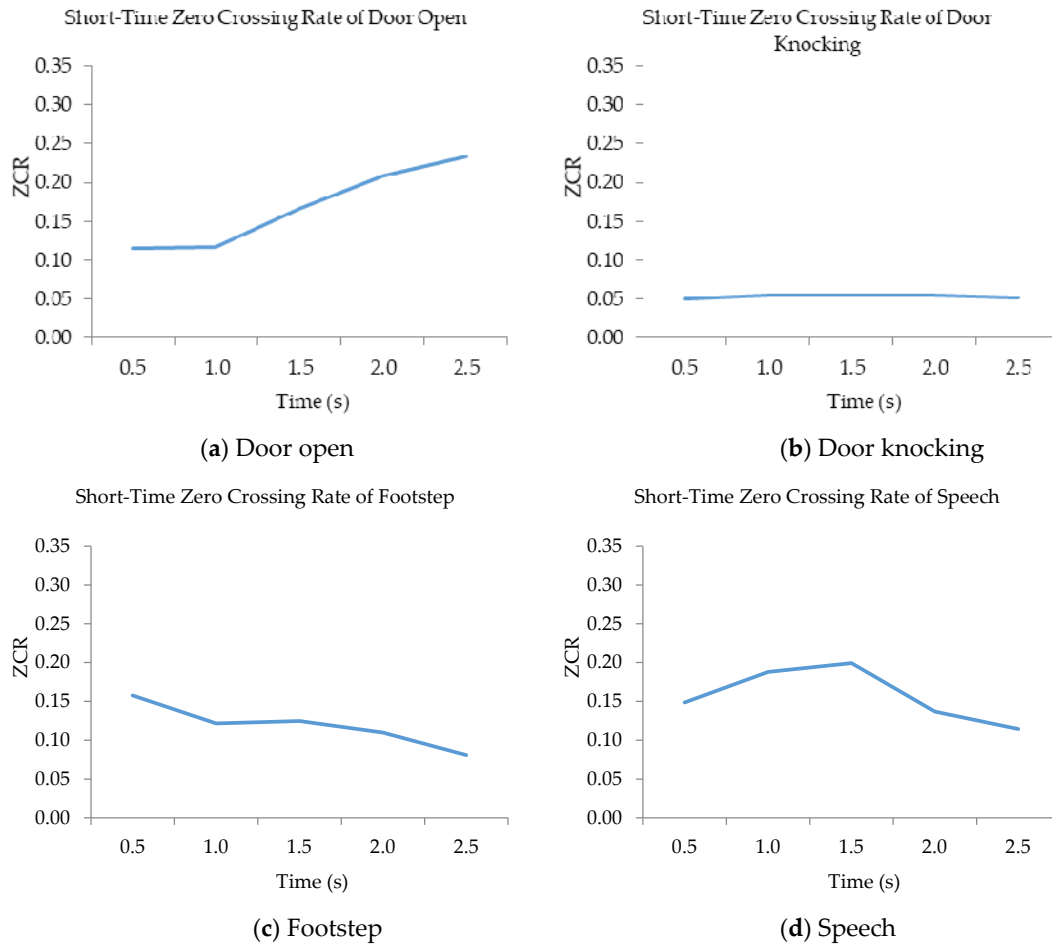
Figure 6. STZCR patterns of four sound-events (a–d).
