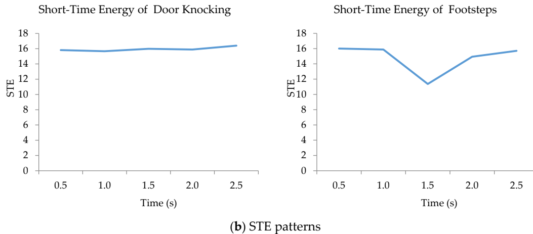
Figure 7. MFCCs (a) and STE (b) patterns of door knocking and footstep.
