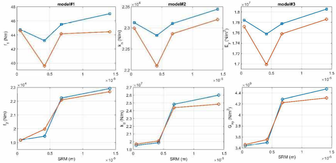
Figure 17. Identified joint model parameters for different contact surface roughness qualities and preloads, (○) P=30 N and (◻) P=50N.
