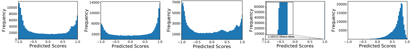
(a) SVM-ALL basic classifier (b) NCWS approach (c) SVM-P approach (d) C-PU approach (e) P-conf approach
