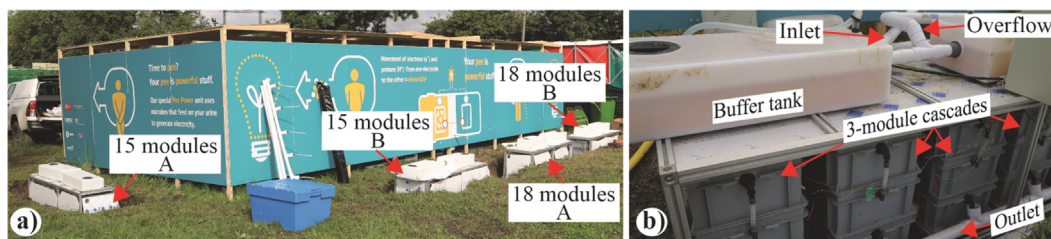
Fig. 3. Pictures illustrating the setup deployed during the field trial. Picture (a) shows how the four stacks were distributed around the back of the 40-person pissoir, which comprised 2 cubicles of 5\text{ m} \times 5\text{ m} . Picture (b) is a close-up of the “15-module B” stack showing the 3-module cascades and the hydraulic connections of the system. (2-column fitting figure).
