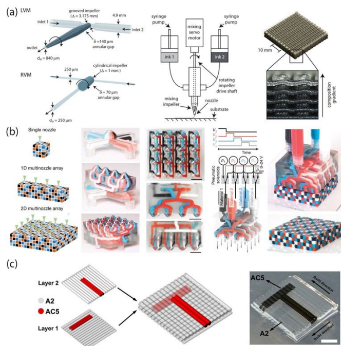
Figure 1. Multi-material 3D printing approaches for soft-materials. (a) Systems for active mixing in situ during printing using rotating impellers (grey shadow) designed for Large (LVM) and Reduced (RVM) volumes. These systems enable the integration of multi-material graded compositions into a structure. Reproduced from ref. 44 with permission from John Wiley and Sons. (b) Multi-material, multi-nozzle 3D printheads in a microfluidic system combining fast pneumatic solenoids and soft inks enable voxelated printing. Reproduced from ref. 42 with permission from Springer Nature. (c) Multi-material deposition of hydrogel structures based on an aspiration-on-demand protocol. The constitutive multi-material segments of extruded filaments were first assembled in liquid state by sequential aspiration of inks into a glass capillary, followed by in situ gel formation. Scale bar (2mm). Reproduced from ref. 46 with permission from Springer Nature.
