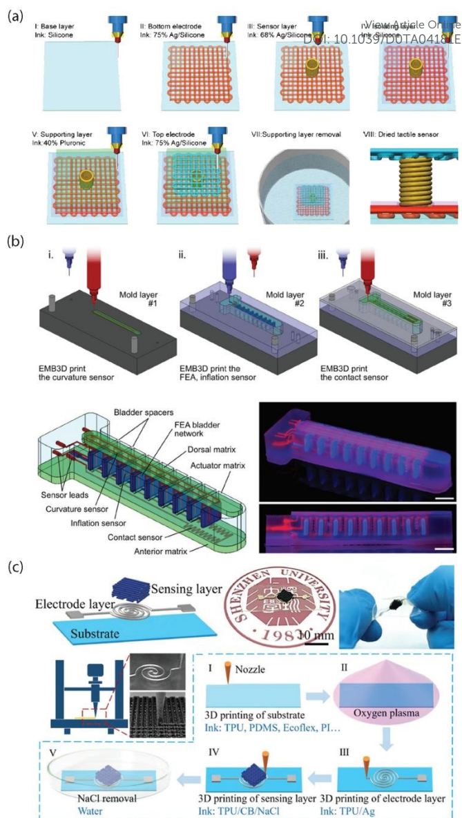
Figure 5. Direct ink writing of multi-material sensor structures. (a) Fabrication of a multilayer tactile sensor using several cartridges and sequential printing; the device is manufactured using Ag/silicone inks with various solid loading fractions for each layer to create the functional components of the sensor (electrodes, sensor, isolation). To print overhanging features, a supporting hydrogel (Pluronic®) layer is used and subsequently removed. Reproduced from ref. 83 with permission from John Wiley and Sons. (b) Somatosensitive actuator featuring multiple soft sensors produced via embedded 3D-printing using a combination of robocasting and moulds; each sensor is produced by printing directly into a matrix material in a mould. Three moulds, with three different matrices (dorsal, actuator, anterior – two-part platinum-cure silicone elastomers of different compositions) are used to host three different components (curvature, inflation, contact – 6 wt% fumed silica in an ionic liquid EMIM-ES). Reproduced from ref. 59 with permission from John Wiley and Sons. (c) Stretchable piezoresistive sensor fabricated by step-by-step printing of a PDMS substrate (cured straight after printing using oxygen
