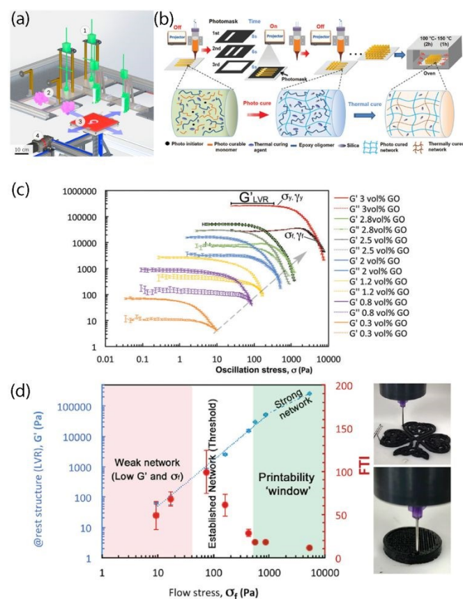
Figure 2. Examples of modified DIW systems (a, b) and criteria for ink printability (c, d). (a) The scheme shows a multi-phase additive manufacturing system that combines DIW components (1) with FDM modules (2) heated platform (3) and with gear-boxes allowing spatial resolution of \pm 3.4 \mu\text{m} (4). Reproduced from ref. 51 with permission from Elsevier. (b) Schematic showing the processes involved in a dynamic photomask-assisted DIW multi-material system. The DIW-printed structure is placed under the dynamic photomask which consists on a projector
