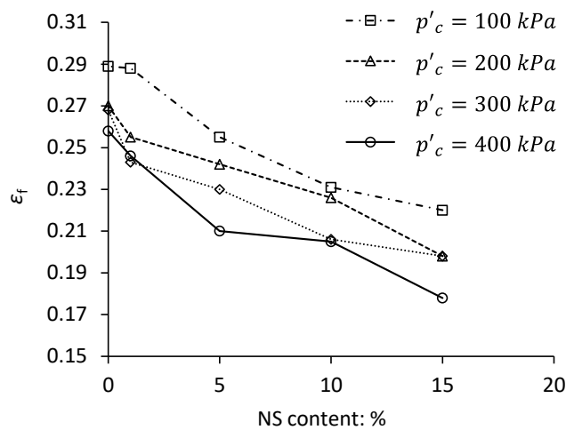
Figure 10. Variation in axial strain at peak deviatoric stress with nano-silica content.
