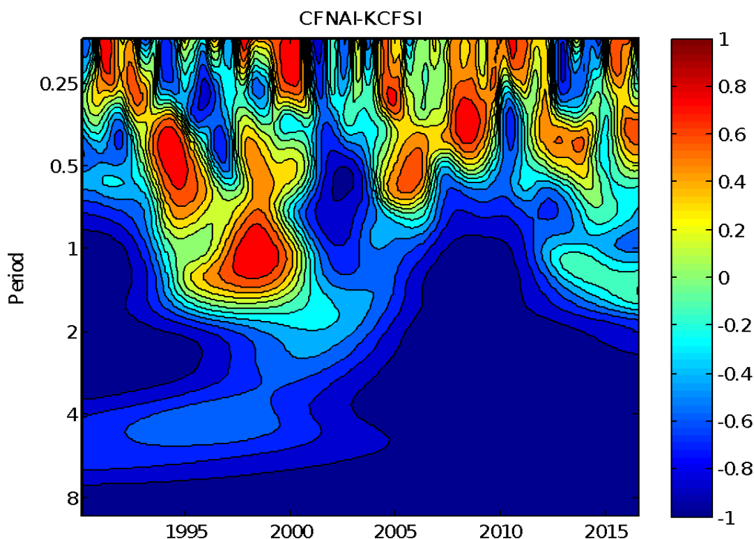
Figure-2: Coherence between economic activity and financial stress
