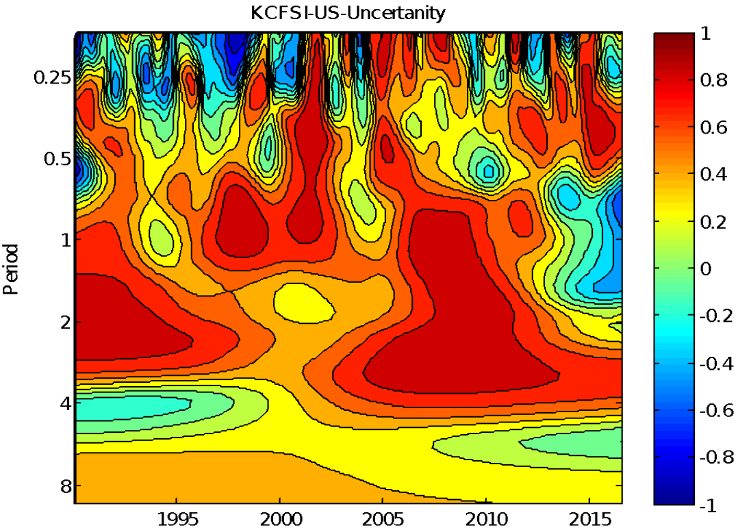
Figure-4: Coherence between financial stress and uncertainty
