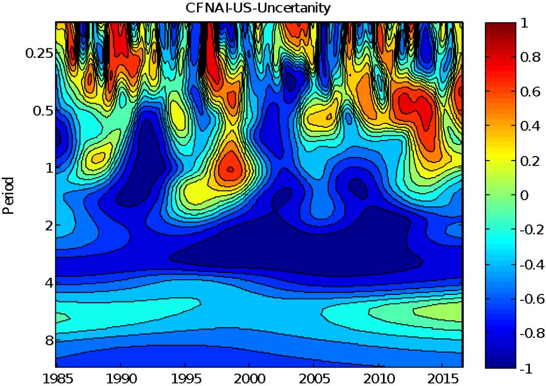
Figure-3: Coherence between economic activity and uncertainty
