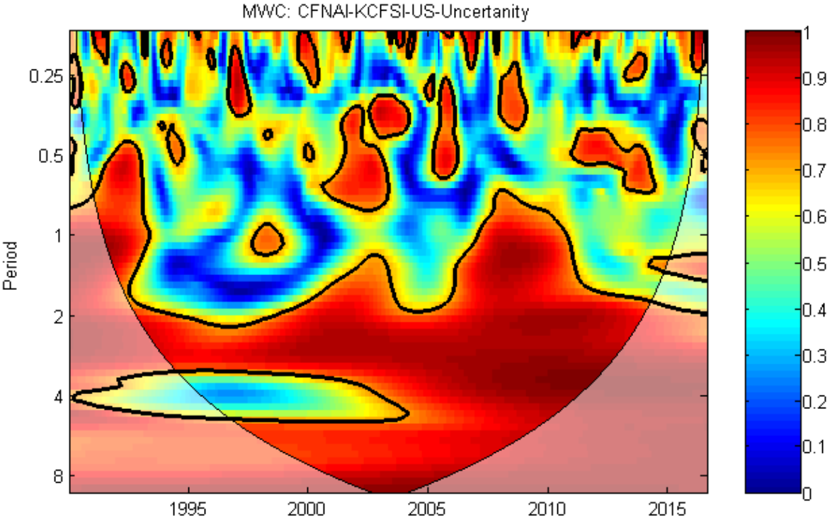
Figure-5: Multiple Wavelet Coherence (MWC) among economic activity, financial stress and uncertainty.
