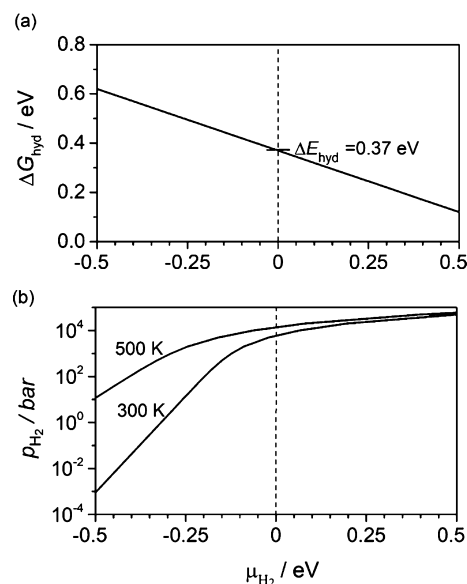
Figure 8. (a) Free energy change involved in hydrogenating an Asp species adsorbed in pentadentate configuration on the Ni{100} surface to form a zwitterionic species adsorbed in tetradentate configuration, from hydrogen in the gas phase, as a function of molecular hydrogen chemical potential; (b) hydrogen partial pressures required to achieve these chemical potentials at 300 and 500 K.
