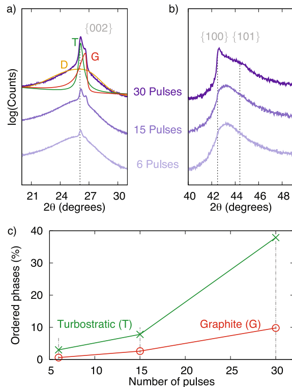
Fig. 5 Analysis of cellulose treated with high-temperature pulses. a Magnification of the \{002\} reflection with the 30-pulse sample showing the disordered (D), turbostratic (T) and graphitic (G) components. b Magnification of the \{100\} and \{101\} reflections with the 30-pulse sample showing the respective components. c Percentage of turbostratic and graphite phases as computed from the intensity ratios of the \{002\} reflection. d HRTEM image of a graphitised region showing the stacked graphitic fringes. e HRTEM image of a classic non-graphitising region.
