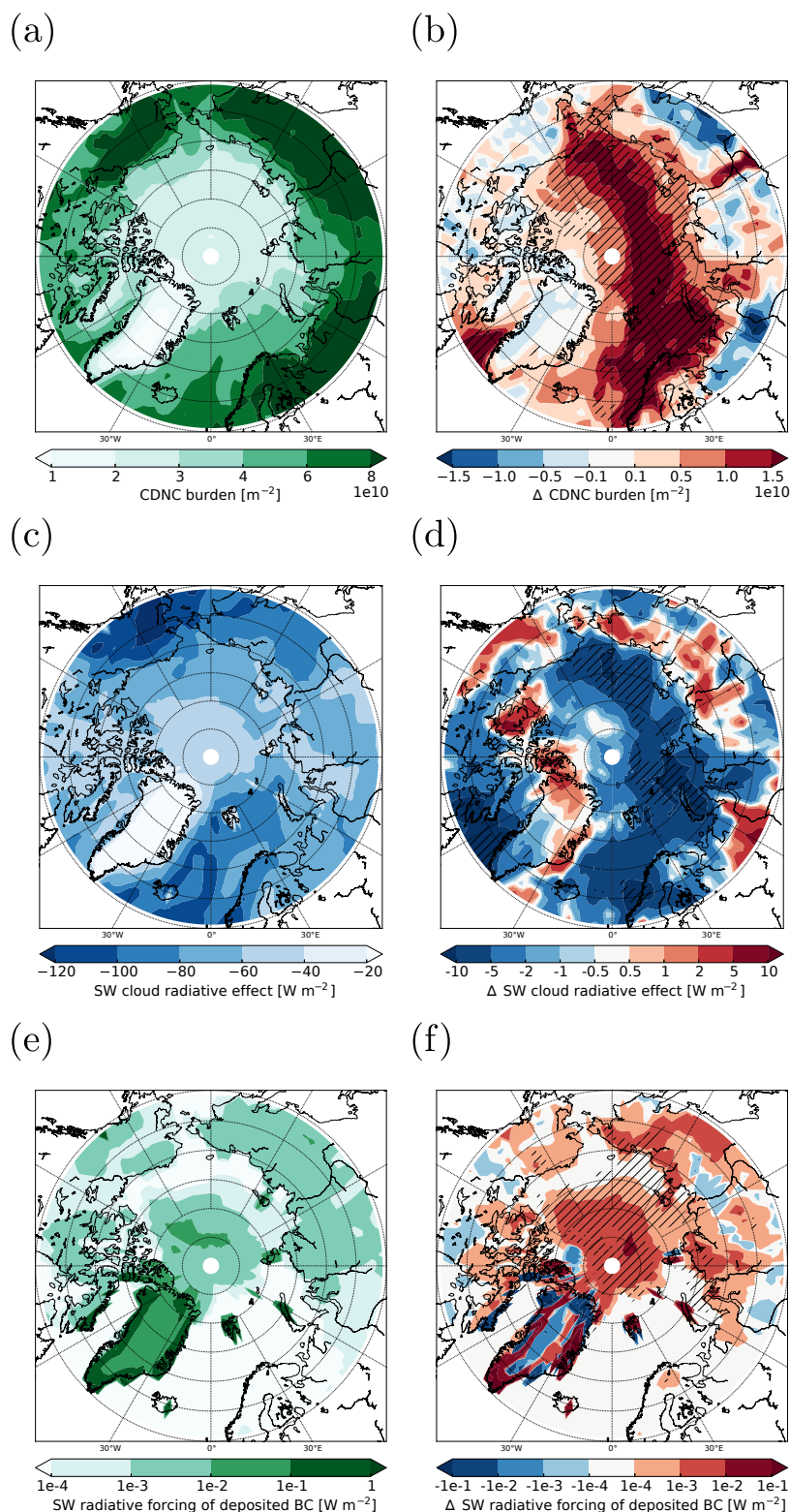
Figure 14. The impact of additional ship emissions in the Arctic on (b) in-cloud CDNC burden, (d) SW CRE, and (f) radiative forcing due to BC deposition on snow. In (a), (c), and (e), the reference without additional ship emissions is shown (arctic_2050). Hatched areas are significant at the 95 % confidence level. Panels (a) to (d) show results for late summer (July–August), (e) and (f) for early autumn (September–October). Note that the scale in (e) and (f) is logarithmic.
