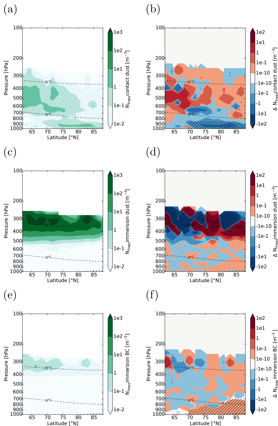
Figure 12. Number of cloud droplets that freeze heterogeneously per time step ( N_{\text{freeze}} ) in 2050: (a, b) contact freezing by dust, (c, d) immersion freezing by dust, (e, f) immersion freezing by black carbon in late summer (July–August). On the left side, absolute values for 2050 (reference) are shown. On the right side, the difference between a simulation with enhanced ship emissions and the reference simulation is displayed (difference between arctic_2050_shipping and arctic_2050). Note that the scale is logarithmic and that the lowest bin had to be decreased to 10^{-10} to display statistically significant increases in immersion freezing by BC. Hatched areas are significant at the 95 % confidence level. The dashed lines show the 0 and the -35 °C isotherms.
