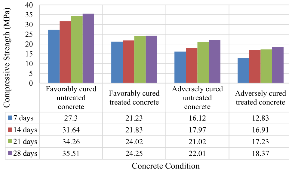
Fig. 7. Compressive strength values for adopted concrete mix under different curing conditions.
