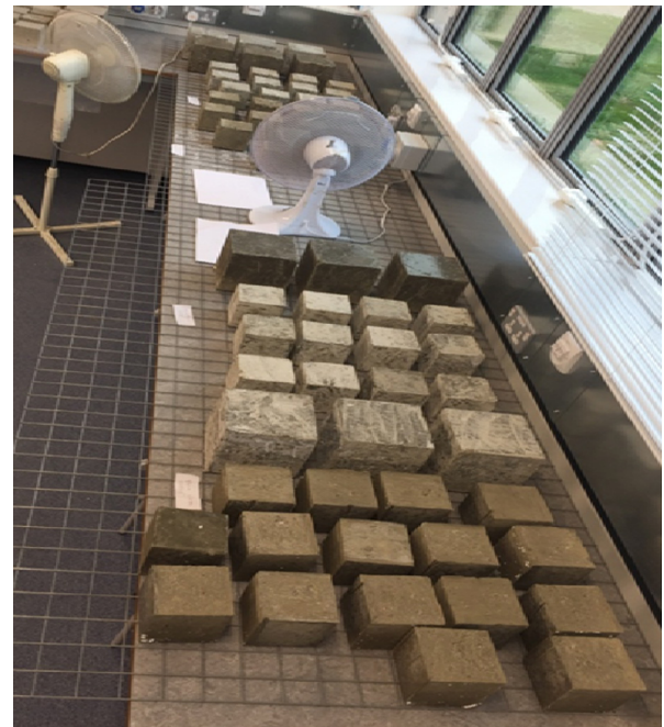
Fig. 2. Treated concrete cubes cured under favorable and adverse conditions.
