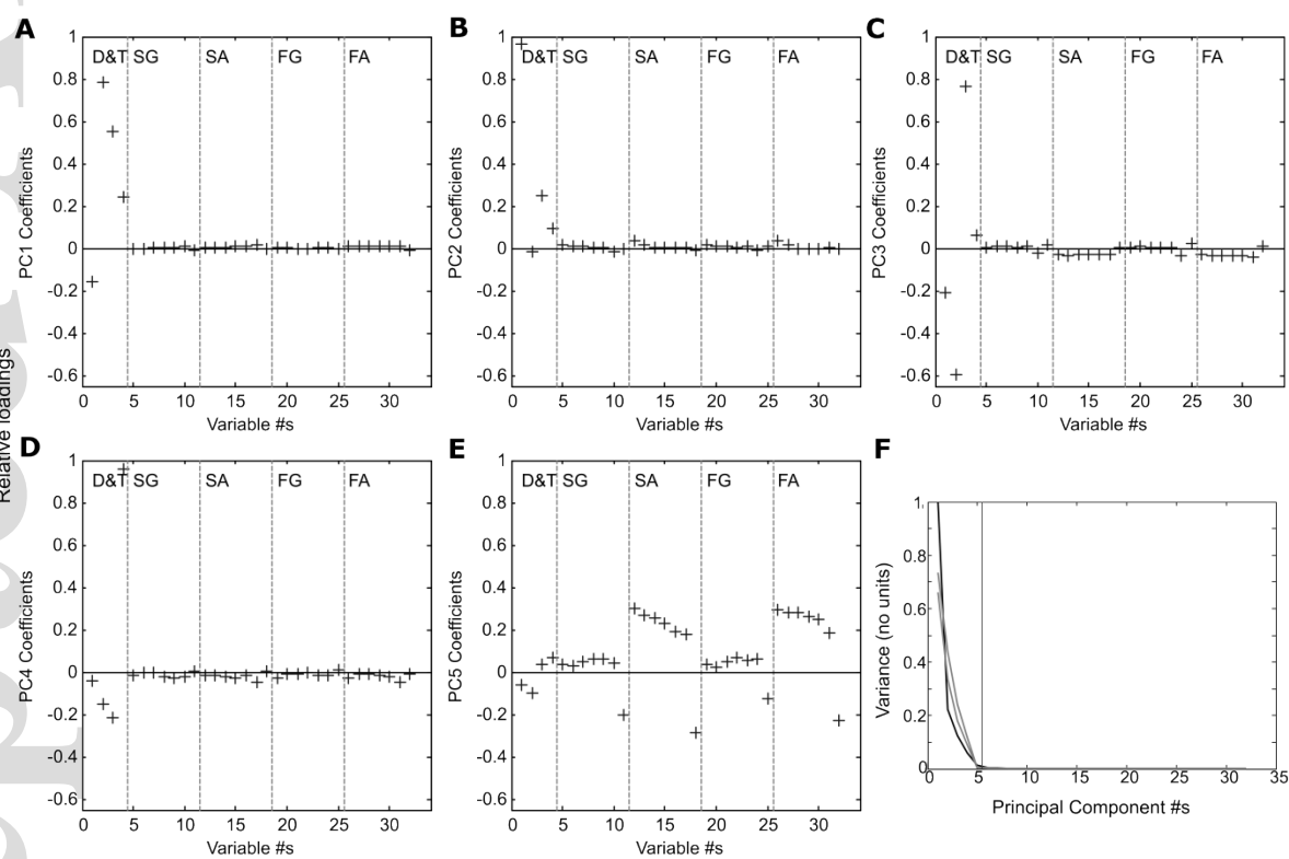
Figure 6: The relative loadings/weights \alpha of each of the variables in PCA space. The numbered variables are detailed in Table 1. A. For PC1: A plot of the relationship between the normalised weights once projected onto PCA space for each variable, compared for the first PCA component. Only the traits/demographics in the first column (#1-4) contribute. B. PC2: Only the demographics/traits (# 1-4) contribute. C. PC3 is dominated by variables #1-4, in particular #3, BAI and there is some relationship with eye movement measures under antigravity. D. PC4 is dominated by #4, GHQ. E. PC5 is dominated by the eye tracking measures, particularly under the antigravity conditions (#12-18 & #26-32) with maximum values around 0.27-0.30, lower than 0.76-0.96 for PC1-4. The strongest
