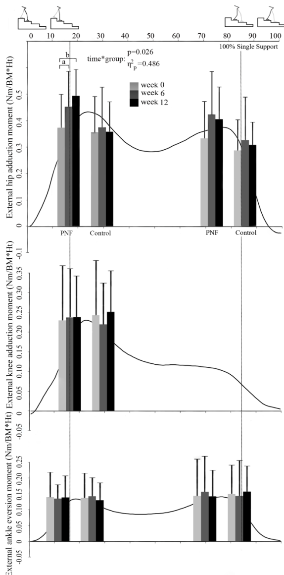
Figure 1. Joint moments of hip, knee and ankle
