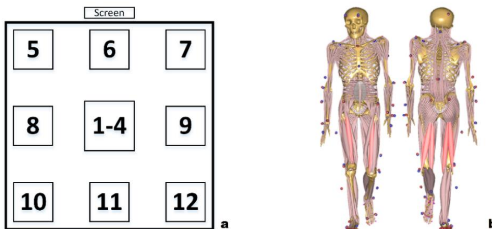
Figure 1: a) Schematic view of the SpeedCourt system with the location and numeration of the pressure sensors. The sensors 1-4 in the middle were treated as one field for this study. b) Musculoskeletal model of the AnyBody Managed Model Repository (AMMR, v. 2.2.0).
