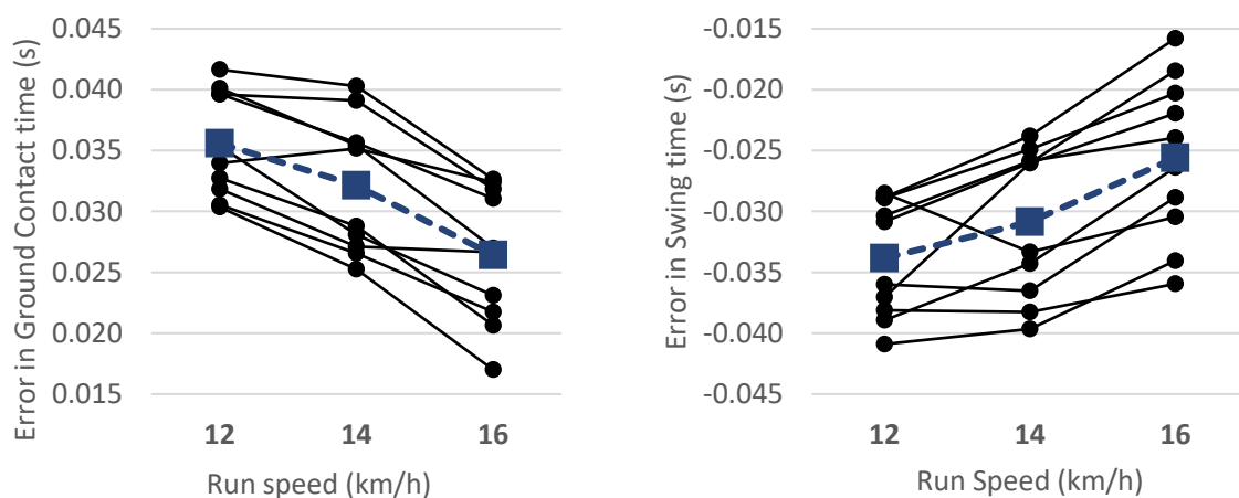
Figure 2: (a) Errors in contact time for 12, 14 and 16 km/h. (b) Errors in swing time for 12, 14 and 16 km/h. Negative values represent underestimation by the Optojump. Averages shown with dashed line.
