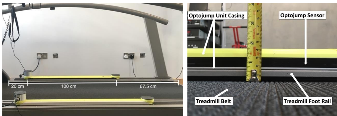
Figure 1: (a) Optojump set-up on the treadmill; (b) Distance between the treadmill belt and the Optojump system.
