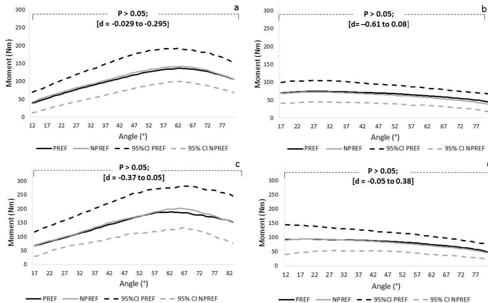
Figure 2. Mean \pm 95%CI moment-angle profiles between PREF and NPREF limbs for concentric; knee extensors (a), knee flexors (b); and eccentric; knee extensors (c), knee flexors (d).
