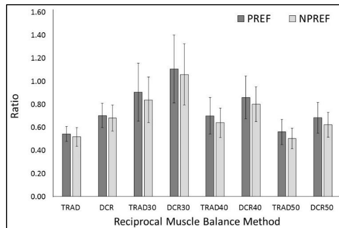
Figure 1: Reciprocal peak moment and angle-specific ratio comparisons between preferred (PREF) and non-preferred (NPREF) limbs. TRAD = traditional; DCR = Dynamic control ratio; TRAD30; DCR30 = ratios at 30°; TRAD40; DCR40 = Ratios at 40°; TRAD50; DCR50 = ratios at 50°.
