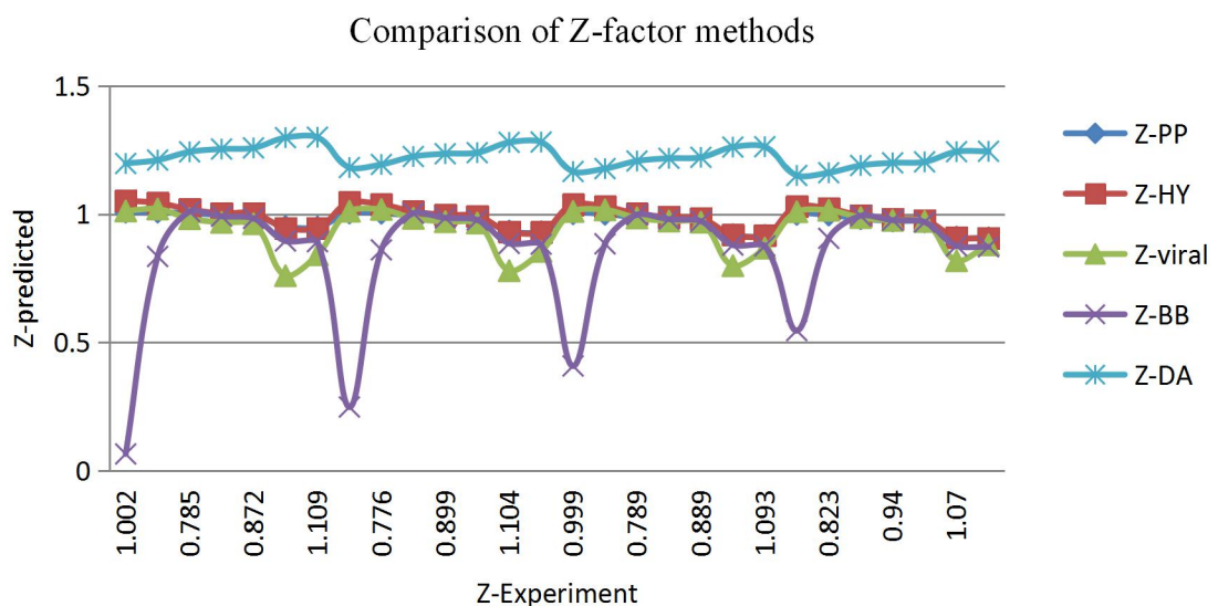
Figure 1: Comparison of the predicted method and the experimental method
