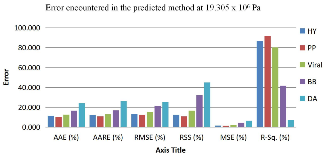
Figure 6: Summary of error in the predicted methods at 19.305*10 6 Pa
