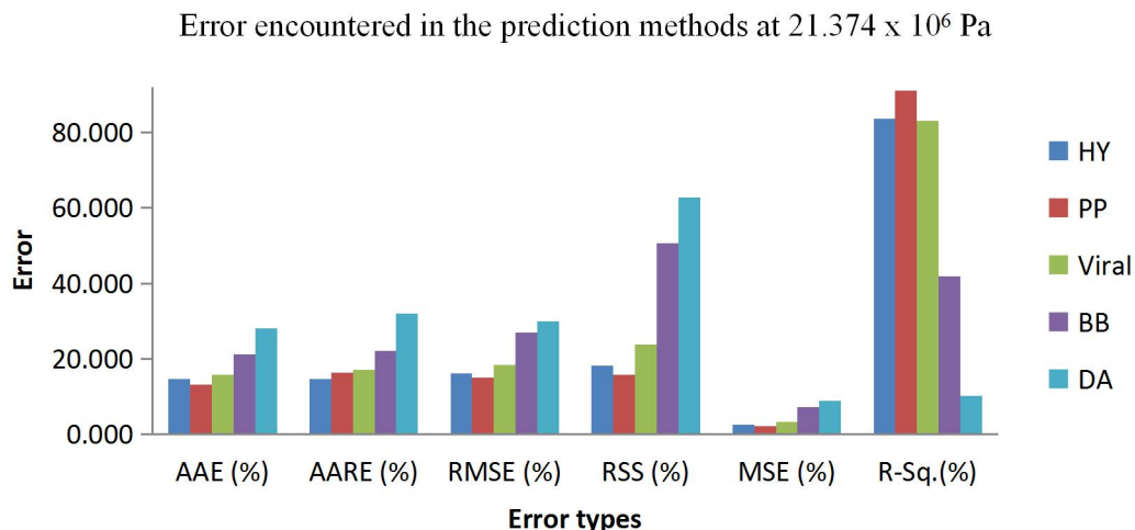
Figure 5: Summary of error in the predicted methods at 21.374*10 6 Pa
