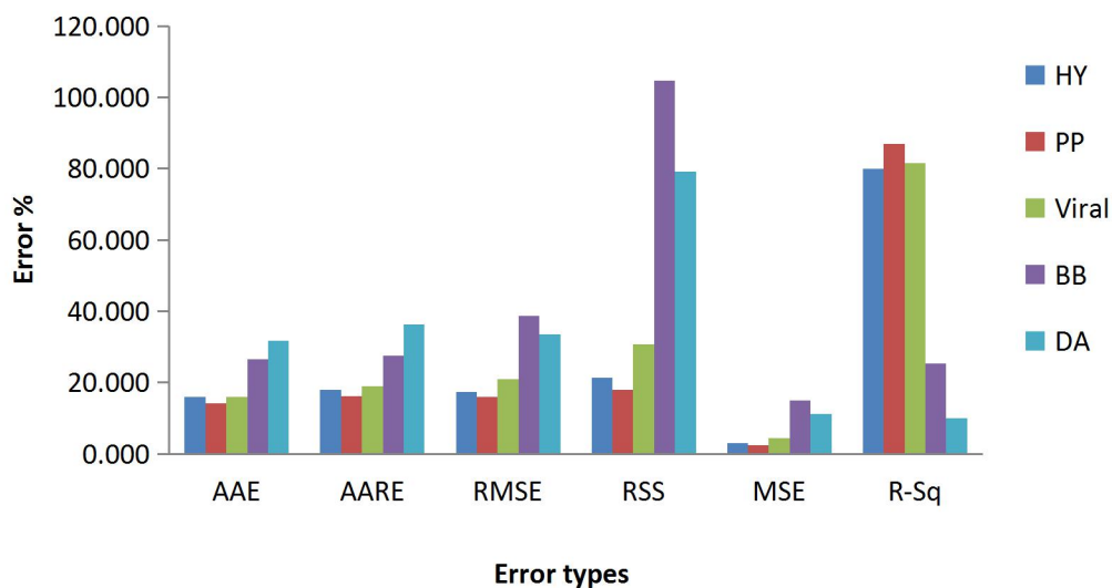
Figure 3: Summary of error in the predicted methods at 25.511 \times 10^6 Pa
