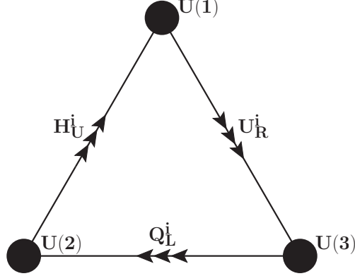
Figure 1: Quiver diagram for D3-branes probing a \mathbb{C}^3/\mathbb{Z}_3 singularity.
